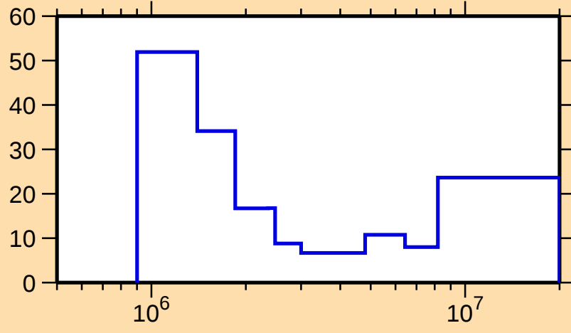
\Delta\sigma/\sigma vs. E for ^{136}\text{Cs}(n,n\text{cont.})
