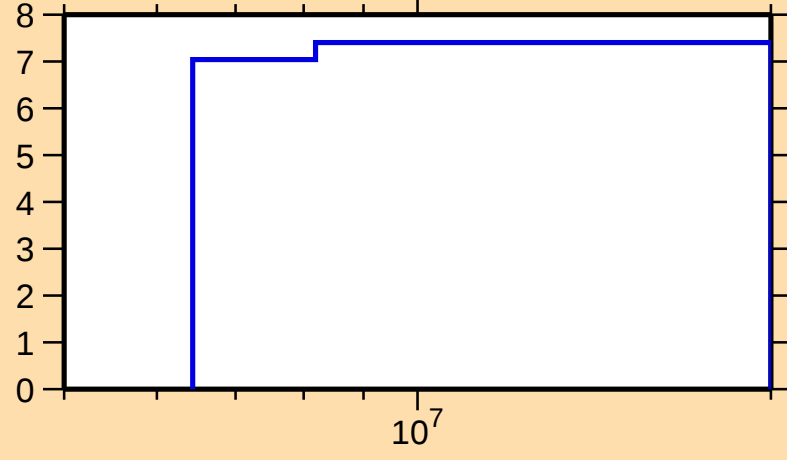
\Delta\sigma/\sigma vs. E for ^{136}\text{Cs}(n,\text{el.})
