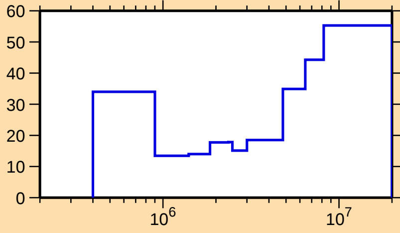
\Delta\sigma/\sigma vs. E for ^{136}\text{Cs}(n,n_1)
