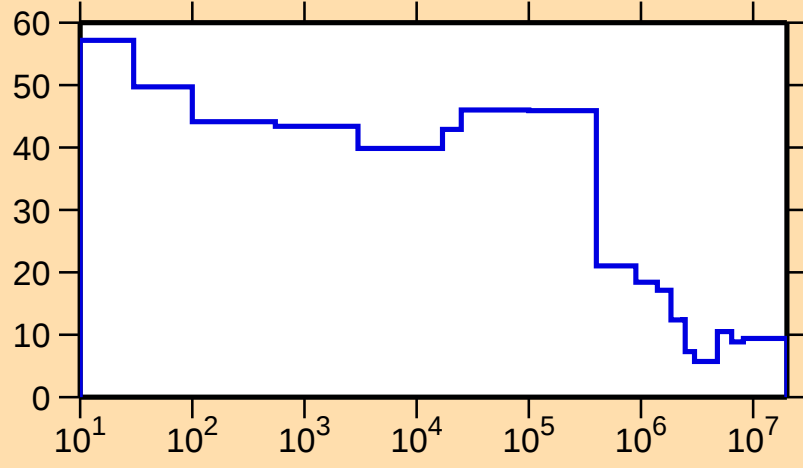
\Delta\sigma/\sigma vs. E for ^{136}\text{Cs}(n,\text{nonel.})
