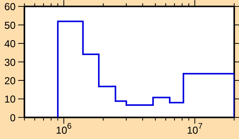
\Delta\sigma/\sigma vs. E for ^{136}\text{Cs}(n,n\text{cont.})
