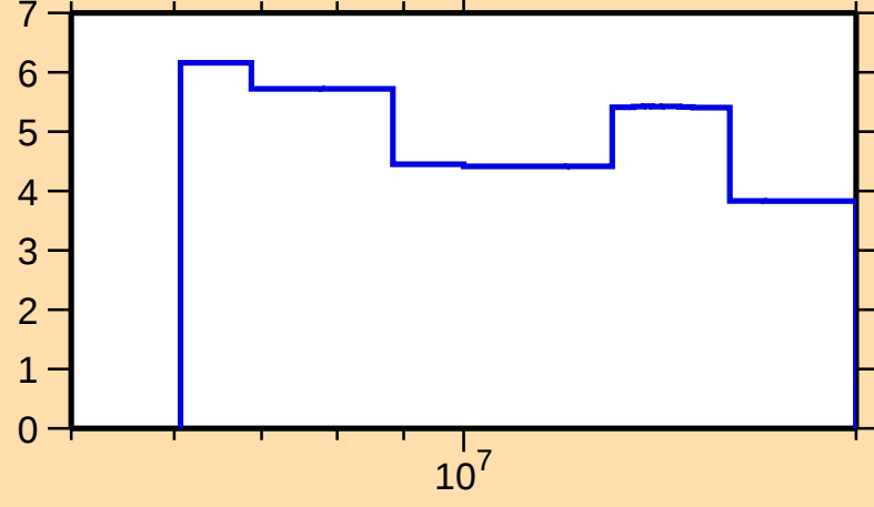
\Delta\sigma/\sigma vs. E for ^{136}\text{Cs}(n,\text{nonel.})
