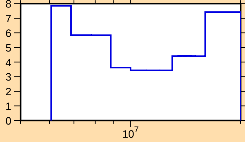
\Delta\sigma/\sigma vs. E for ^{136}\text{Cs}(n,\text{tot.})
