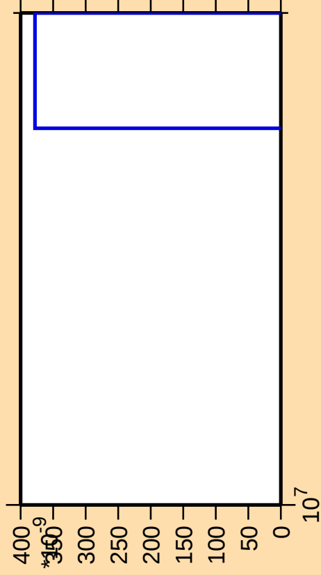
\Delta\sigma/\sigma vs. E for ^{136}\text{Cs}(\text{mt 11})
