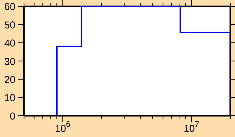
\Delta\sigma/\sigma vs. E for ^{136}\text{Cs}(n,p)
