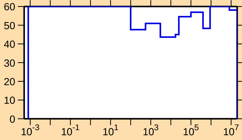
\Delta\sigma/\sigma vs. E for ^{136}\text{Cs}(n,\gamma)
