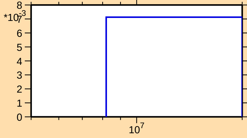
\sigma vs. E for ^{136}\text{Cs}(n,3n)
