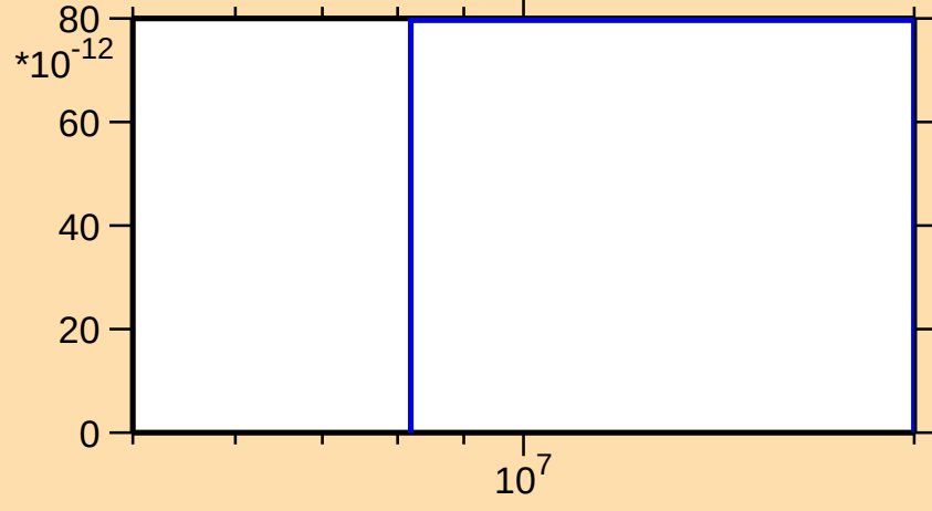
\sigma vs. E for ^{136}\text{Cs}(n,2n\alpha)
