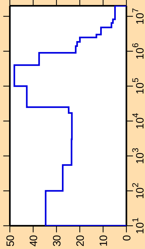
\Delta\sigma/\sigma vs. E for ^{136}\text{Cs}(n,\text{nonel.})
