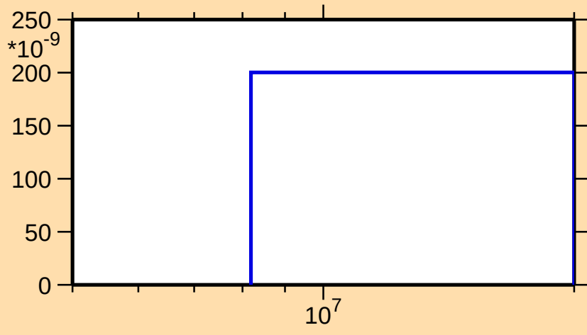
\sigma vs. E for ^{136}\text{Cs}(n,\text{nd})
