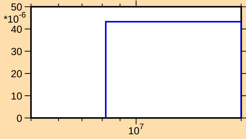
\sigma vs. E for ^{136}\text{Cs}(n,n\alpha)
