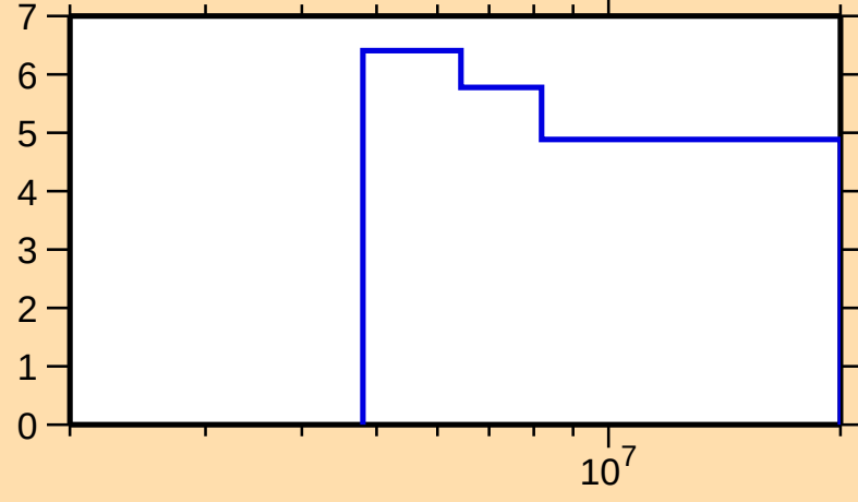
\Delta\sigma/\sigma vs. E for ^{136}\text{Cs}(n,\text{nonel.})
