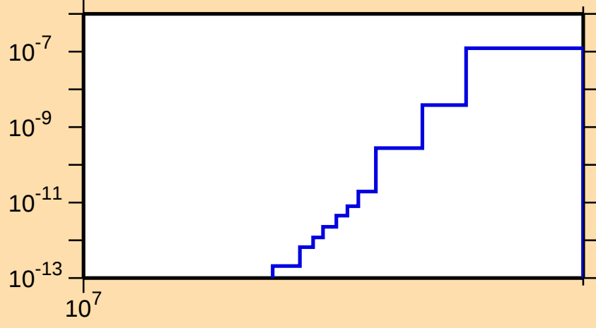
\sigma vs. E for ^{138}\text{Cs}(n,2n\alpha)
