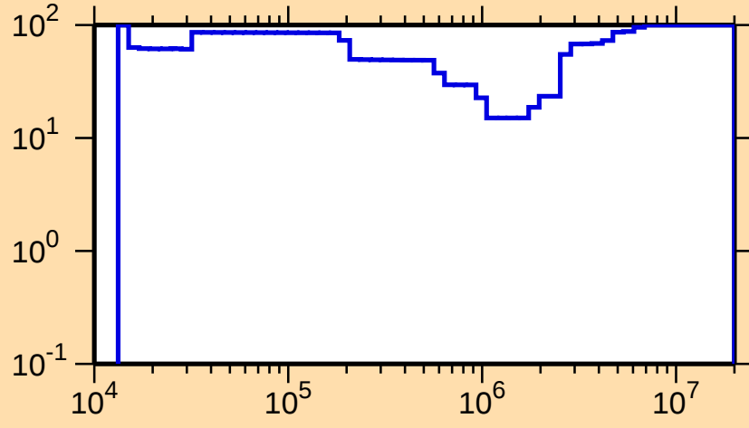
\Delta\sigma/\sigma vs. E for ^{138}\text{Cs}(n,n_1)
