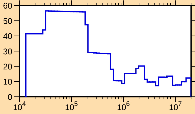
\Delta\sigma/\sigma vs. E for ^{138}\text{Cs}(n,\text{el.})
