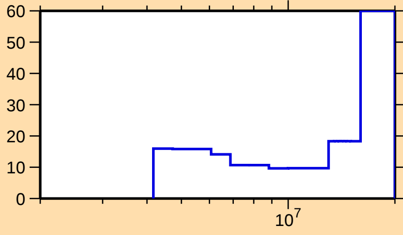
\Delta\sigma/\sigma vs. E for ^{138}\text{Cs}(n,2n)
