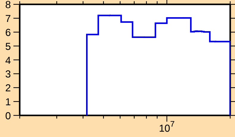
\Delta\sigma/\sigma vs. E for ^{138}\text{Cs}(n,\text{nonel.})
