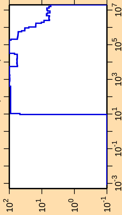
\Delta\sigma/\sigma vs. E for ^{138}\text{Cs}(n,\text{nonel.})
