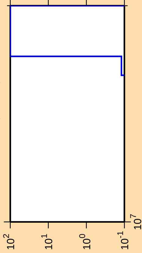
\Delta\sigma/\sigma vs. E for ^{138}\text{Cs}(n,\text{He}3)
