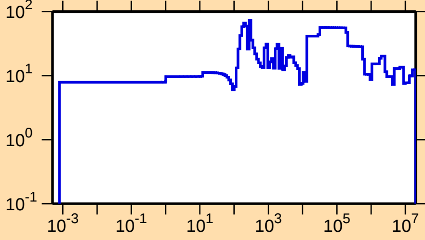
\Delta\sigma/\sigma vs. E for ^{138}\text{Cs}(n,\text{el.})
