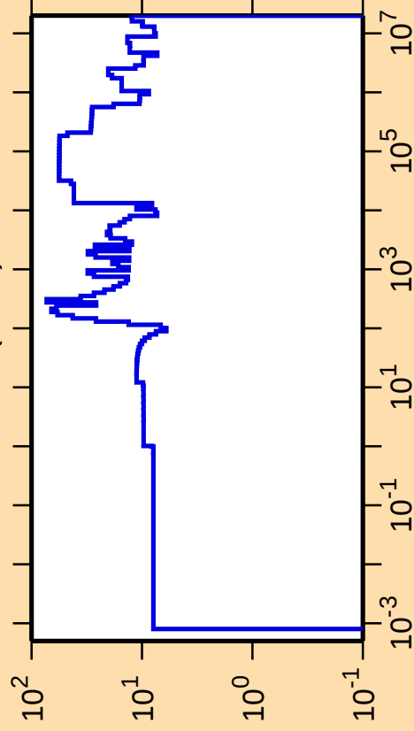
\Delta\sigma/\sigma vs. E for ^{138}\text{Cs}(n,\text{el.})
