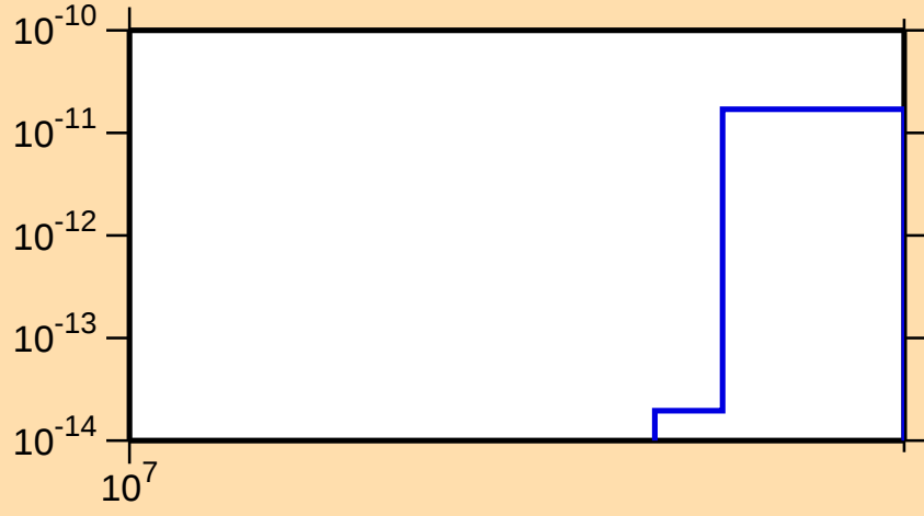
\sigma vs. E for ^{138}\text{Cs}(n,\text{He}3)
