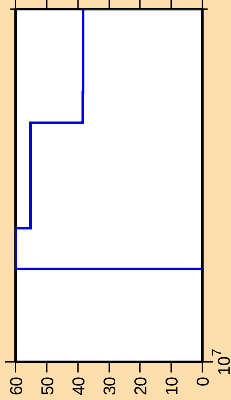
\Delta\sigma/\sigma vs. E for ^{138}\text{Cs}(n,3n)
