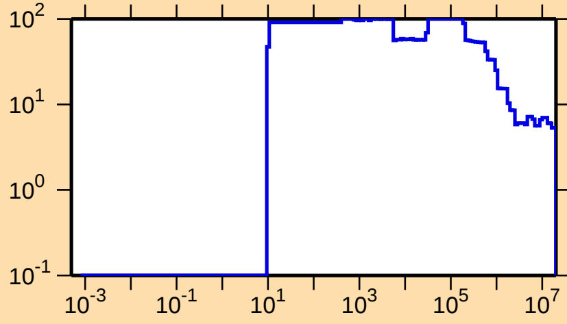
\Delta\sigma/\sigma vs. E for ^{138}\text{Cs}(n,\text{nonel.})
