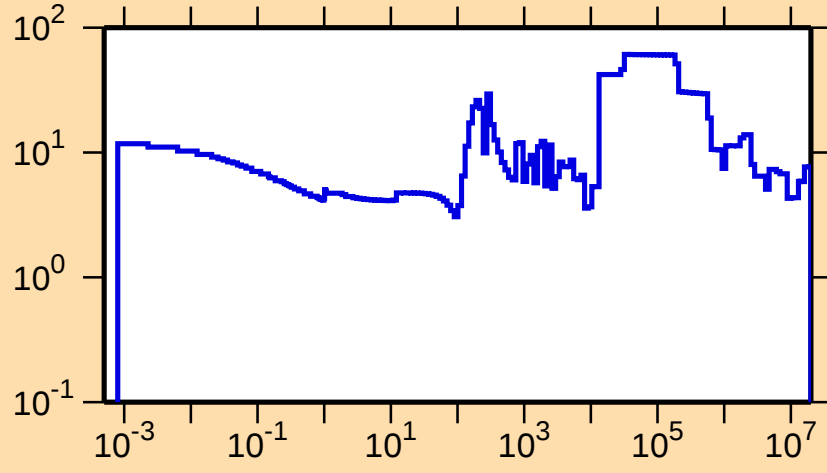
\Delta\sigma/\sigma vs. E for ^{138}\text{Cs}(n,\text{tot.})
