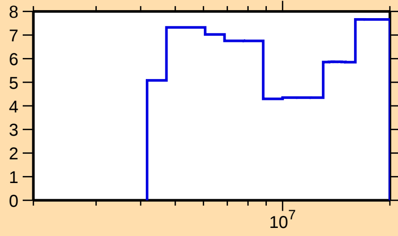
\Delta\sigma/\sigma vs. E for ^{138}\text{Cs}(n,\text{tot.})
