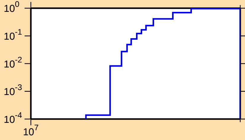
\sigma vs. E for ^{138}\text{Cs}(n,3n)
