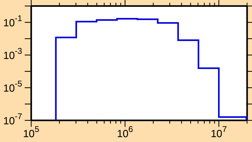
\sigma vs. E for ^{138}\text{Cs}(n,n_4)
