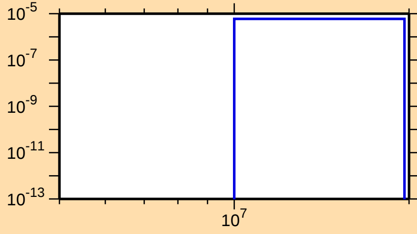
\sigma vs. E for ^{138}\text{Cs}(n,\text{nd})
