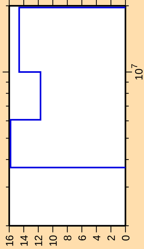
\Delta\sigma/\sigma vs. E for ^{138}\text{Cs}(n,2n)
