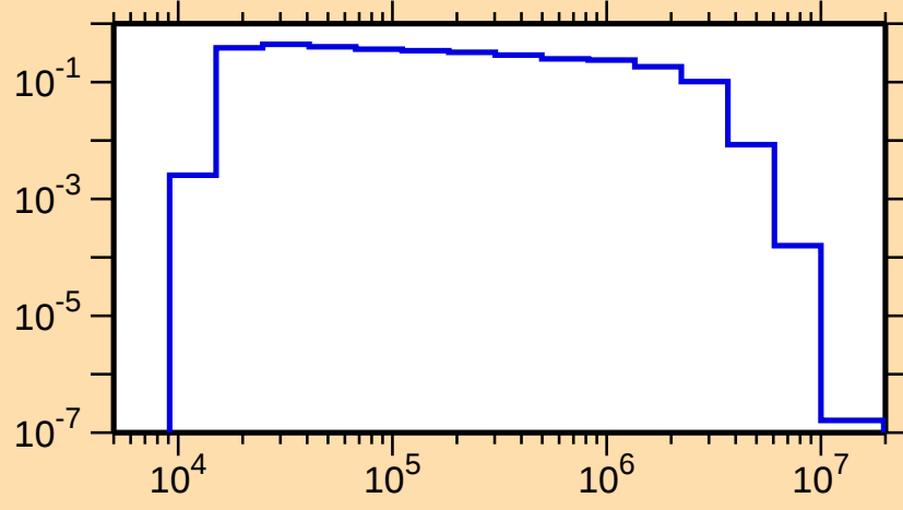
\sigma vs. E for ^{138}\text{Cs}(n,n_1)
