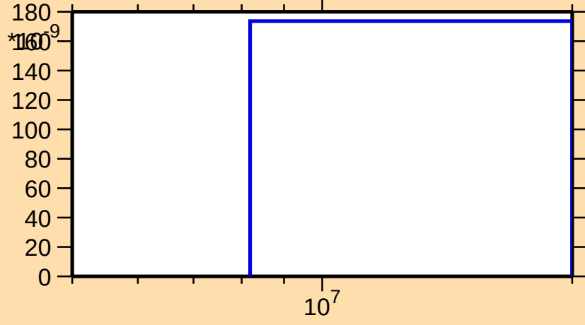
\sigma vs. E for ^{138}\text{Cs}(n,nt)
