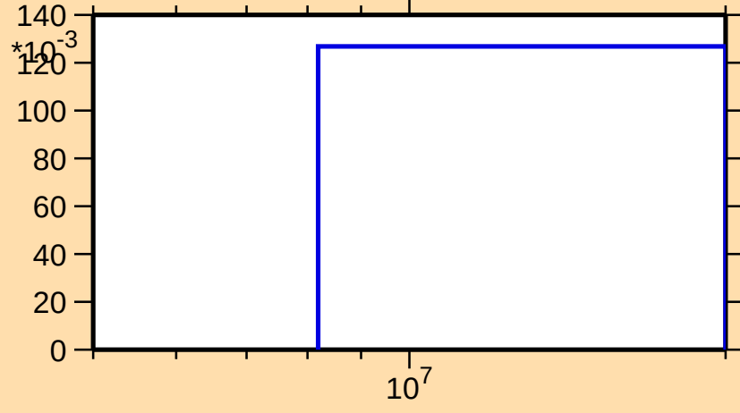
\sigma vs. E for ^{138}\text{Cs}(n,3n)
