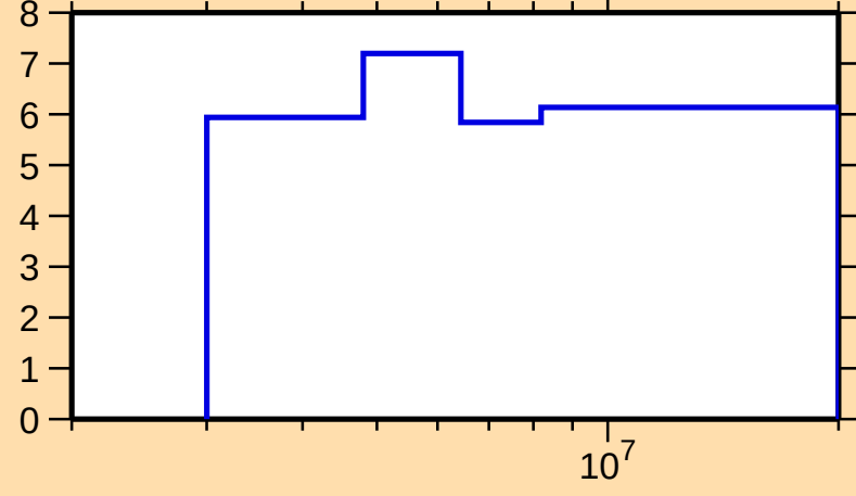
\Delta\sigma/\sigma vs. E for ^{138}\text{Cs}(n,\text{nonel.})
