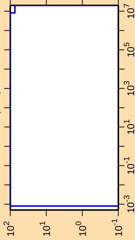
\Delta\sigma/\sigma vs. E for ^{138}\text{Cs}(n,\alpha)
