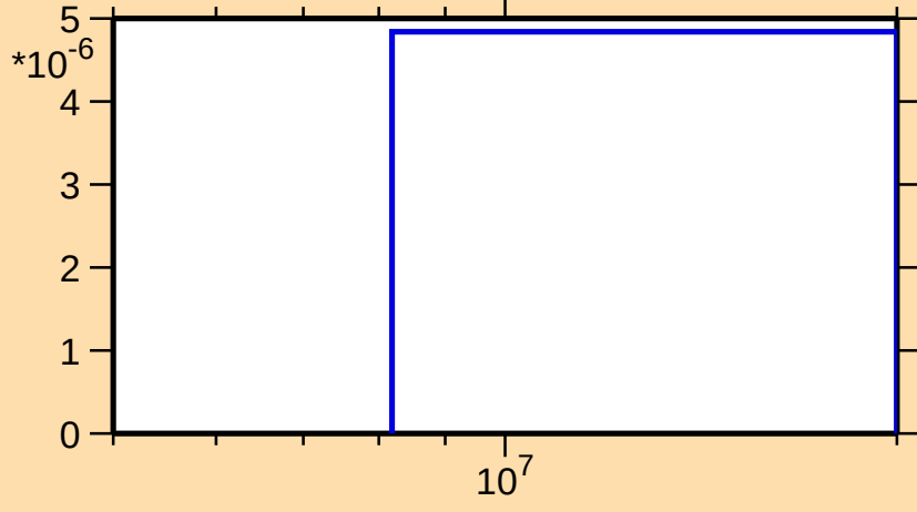
\sigma vs. E for ^{138}\text{Cs}(n,\text{nd})
