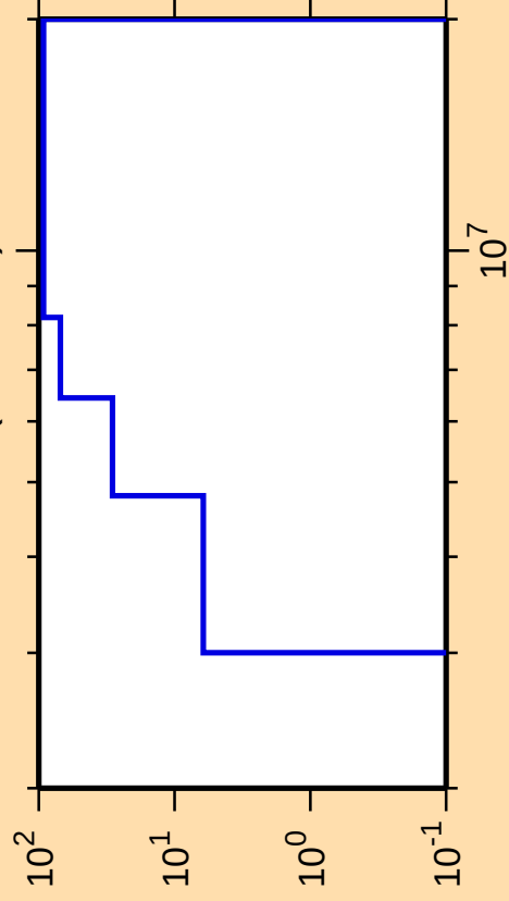
\Delta\sigma/\sigma vs. E for ^{138}\text{Cs}(n,n\text{cont.})
