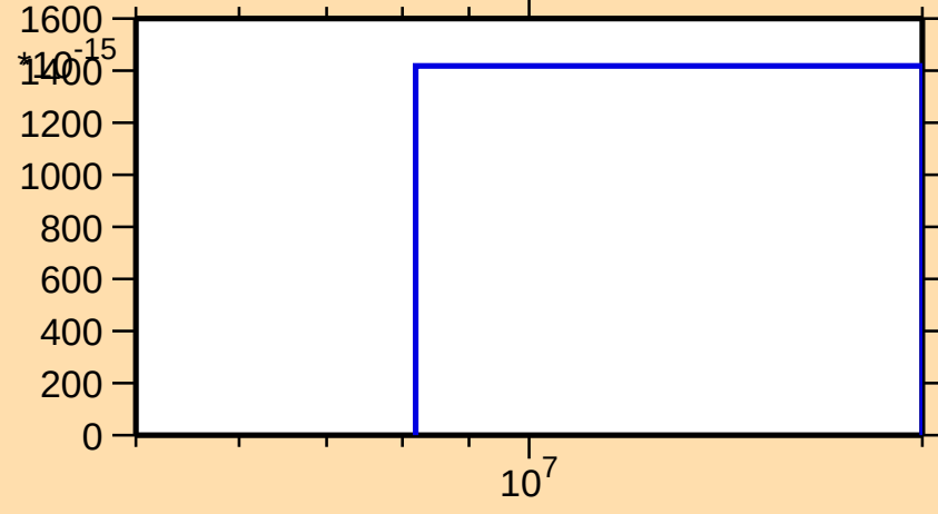
\sigma vs. E for ^{138}\text{Cs}(n,p\alpha)
