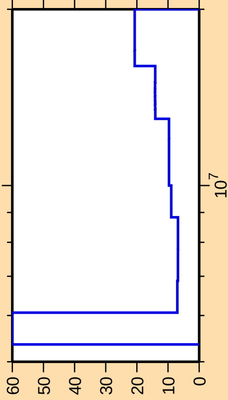
\Delta\sigma/\sigma vs. E for ^{139}\text{Cs}(n,2n)
