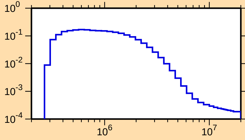
\sigma vs. E for ^{139}\text{Cs}(n,n_2)
