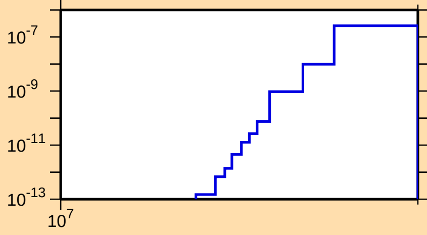
\sigma vs. E for ^{139}\text{Cs}(n,2n\alpha)
