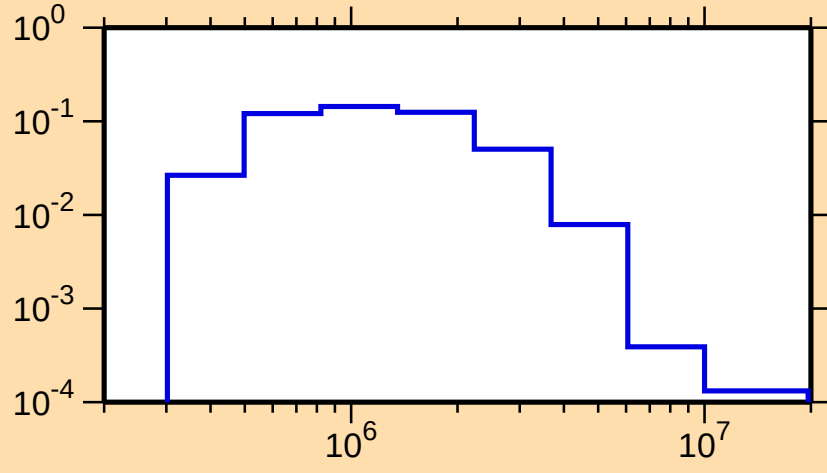
\sigma vs. E for ^{139}\text{Cs}(n,n_3)
