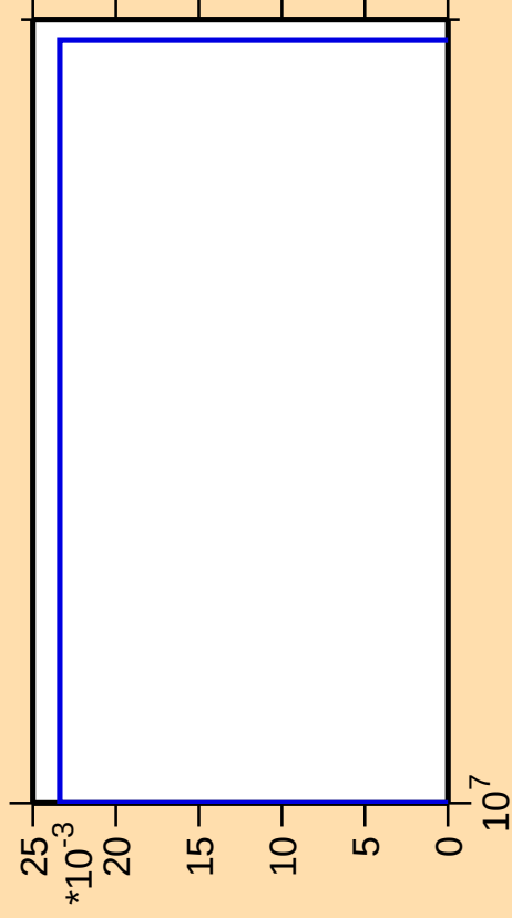
\Delta\sigma/\sigma vs. E for ^{139}\text{Cs}(n,p\alpha)
