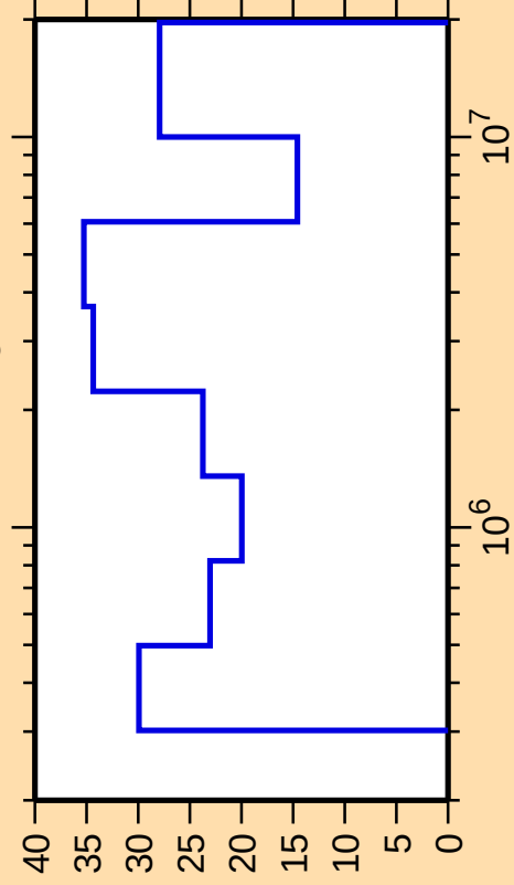
\Delta\sigma/\sigma vs. E for ^{139}\text{Cs}(n,n_3)
