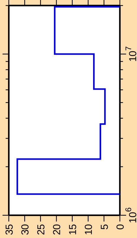
\Delta\sigma/\sigma vs. E for ^{139}\text{Cs}(n,n\text{cont.})
