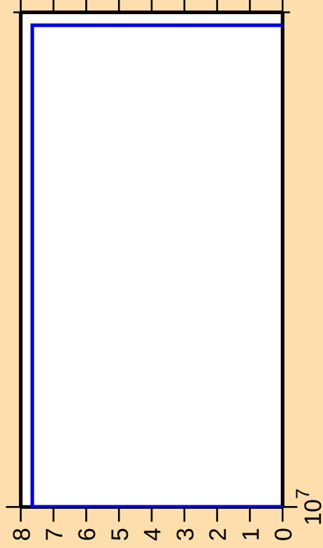
\Delta\sigma/\sigma vs. E for ^{139}\text{Cs}(n,3n)
