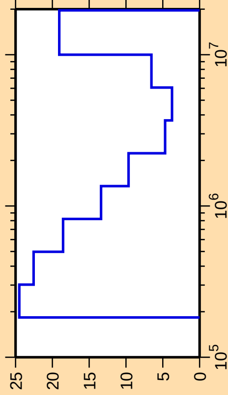
\Delta\sigma/\sigma vs. E for ^{139}\text{Cs}(n,\text{inel.})
