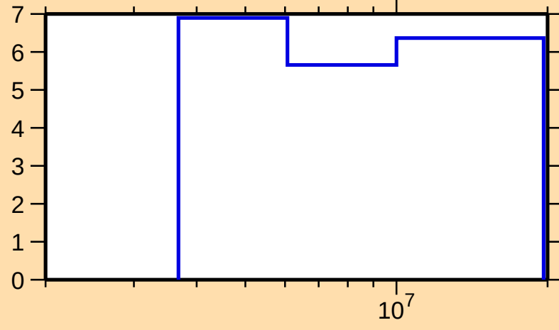
\Delta\sigma/\sigma vs. E for ^{139}\text{Cs}(n,\text{el.})
