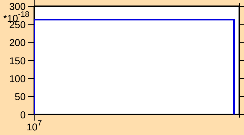
\sigma vs. E for ^{139}\text{Cs} (mt 42)
