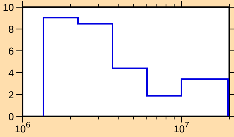
\Delta\sigma/\sigma vs. E for ^{139}\text{Cs}(n,\text{tot.})
