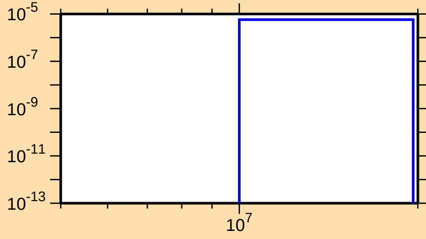
\sigma vs. E for ^{139}\text{Cs}(n,nt)
