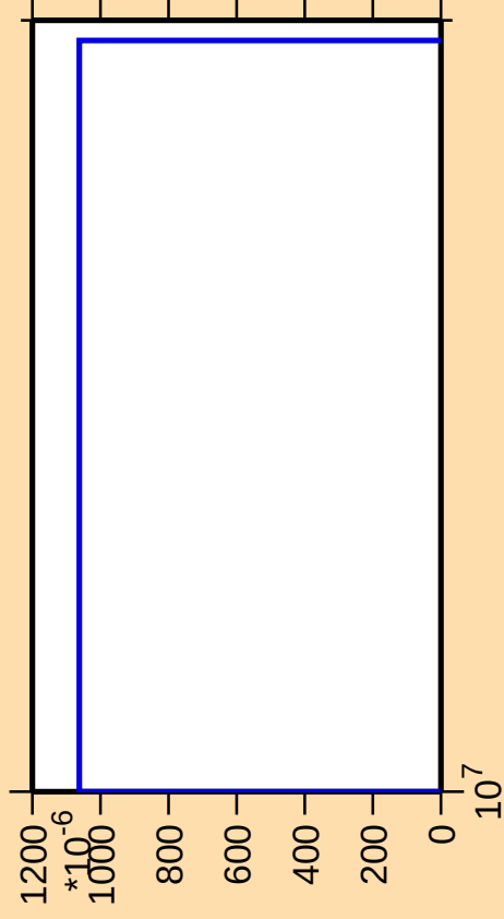
\Delta\sigma/\sigma vs. E for ^{139}\text{Cs} (mt 42)
