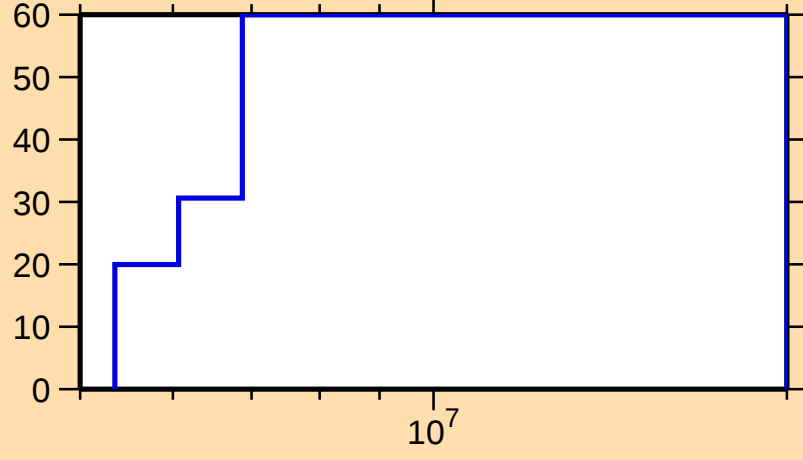
\Delta\sigma/\sigma vs. E for ^{141}\text{Cs}(n,\text{inel.})
