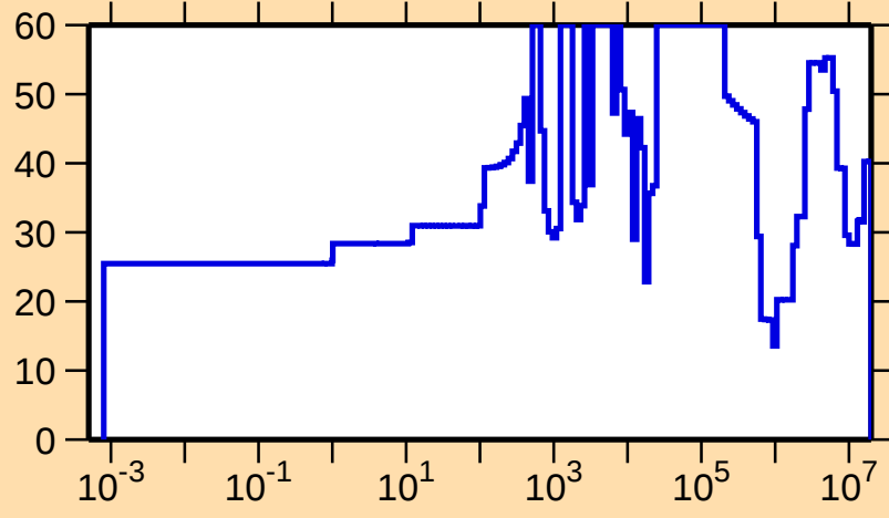
\Delta\sigma/\sigma vs. E for ^{141}\text{Cs}(n,\text{el.})
