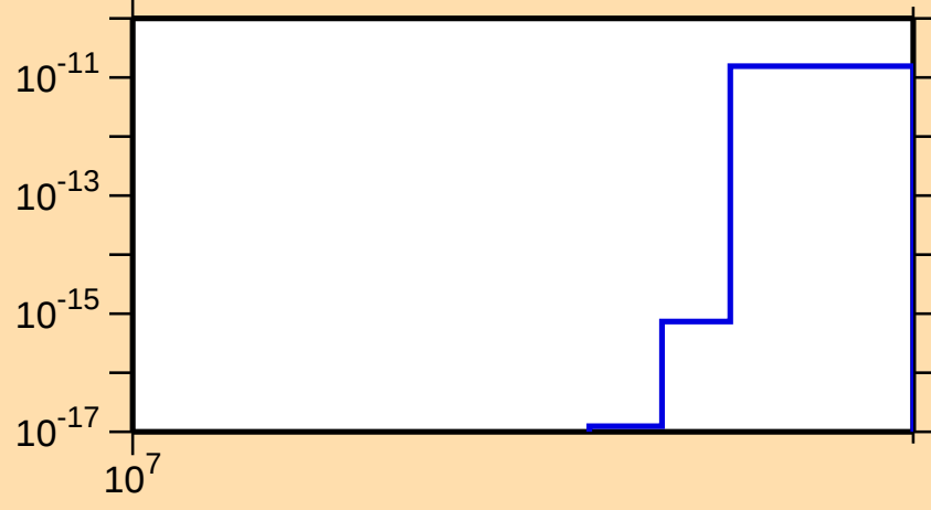
\sigma vs. E for ^{141}\text{Cs} (mt 11)
