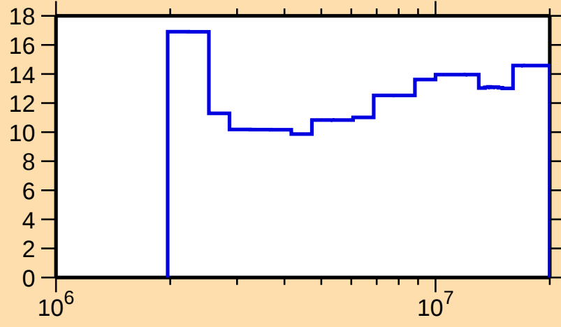
\Delta\sigma/\sigma vs. E for ^{141}\text{Cs}(n,\text{nonel.})
