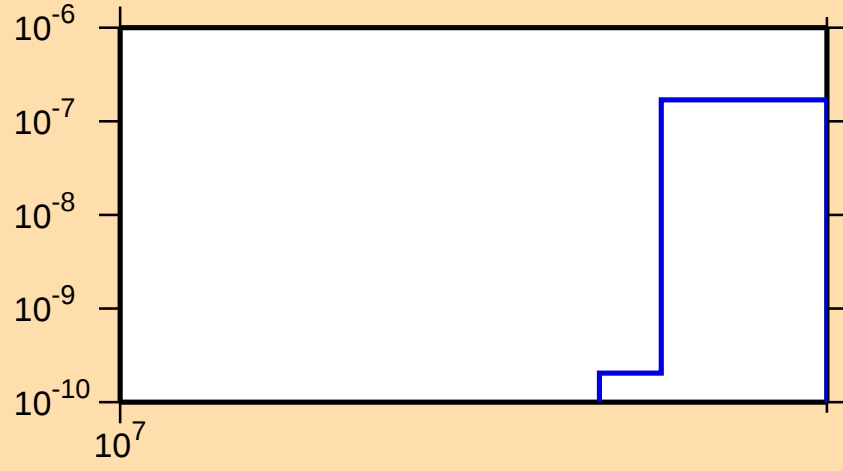
\sigma vs. E for ^{141}\text{Cs}(n,2np)
