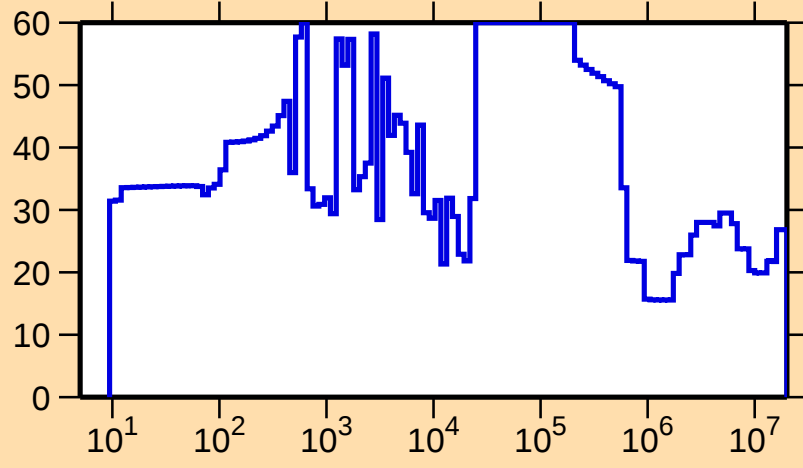
\Delta\sigma/\sigma vs. E for ^{141}\text{Cs}(n,\text{tot.})
