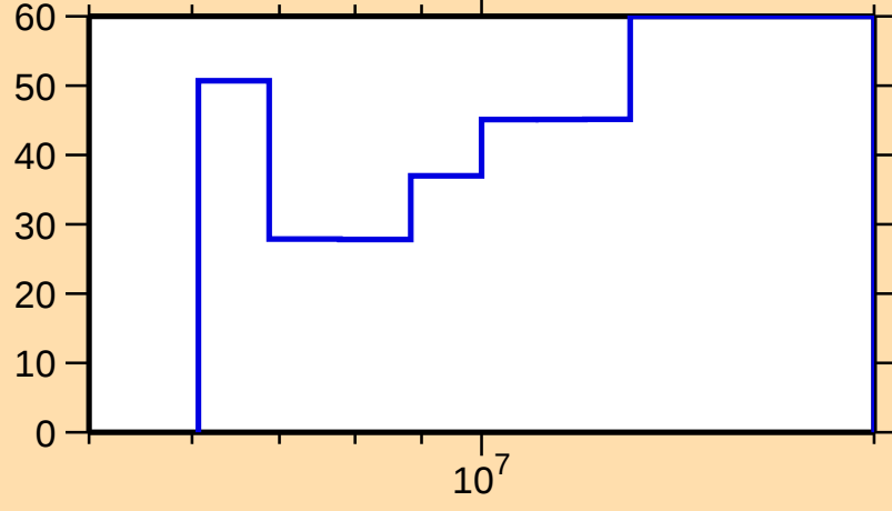
\Delta\sigma/\sigma vs. E for ^{141}\text{Cs}(n,2n)
