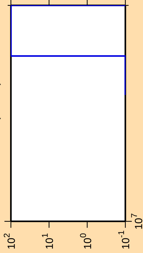
\Delta\sigma/\sigma vs. E for ^{141}\text{Cs} (mt 11)
