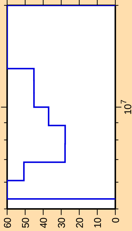
\Delta\sigma/\sigma vs. E for ^{141}\text{Cs}(n,2n)
