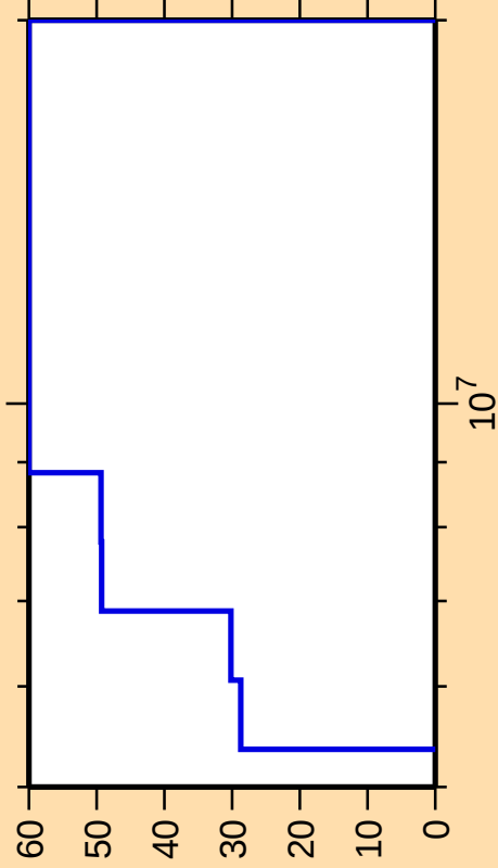
\Delta\sigma/\sigma vs. E for ^{141}\text{Cs}(n,n\text{cont.})
