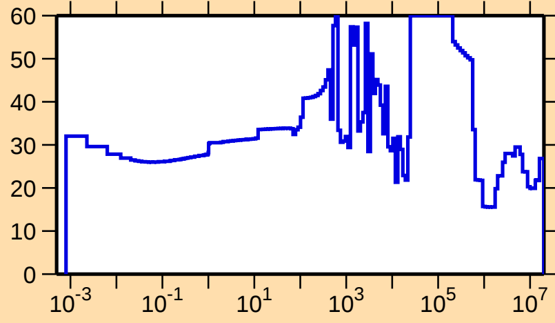
\Delta\sigma/\sigma vs. E for ^{141}\text{Cs}(n,\text{tot.})
