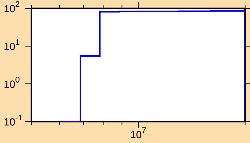
\Delta\sigma/\sigma vs. E for ^{141}\text{Cs}(n,p)
