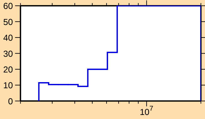
\Delta\sigma/\sigma vs. E for ^{141}\text{Cs}(n,\text{inel.})
