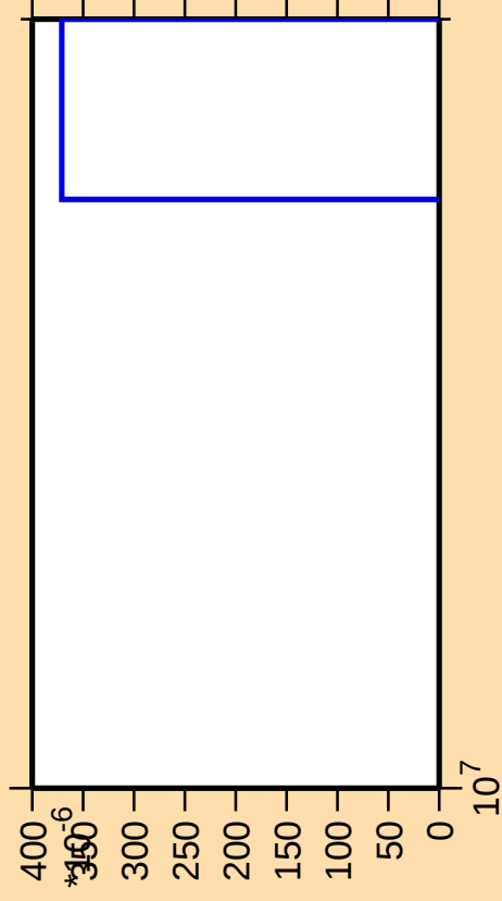
\Delta\sigma/\sigma vs. E for ^{141}\text{Cs} (mt 42)
