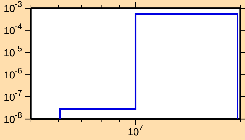
\sigma vs. E for ^{141}\text{Cs}(n,p)
