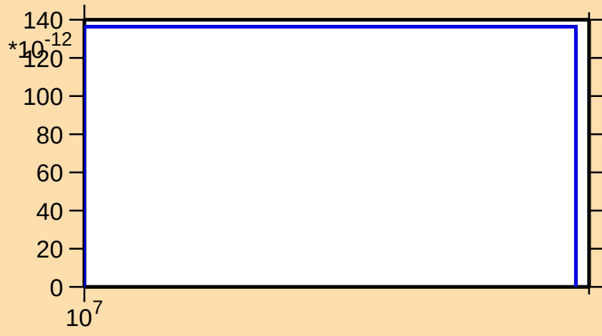
\sigma vs. E for ^{141}\text{Cs}(n,3n\alpha)
