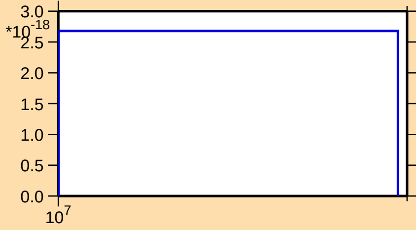
\sigma vs. E for ^{141}\text{Cs} (mt 42)
