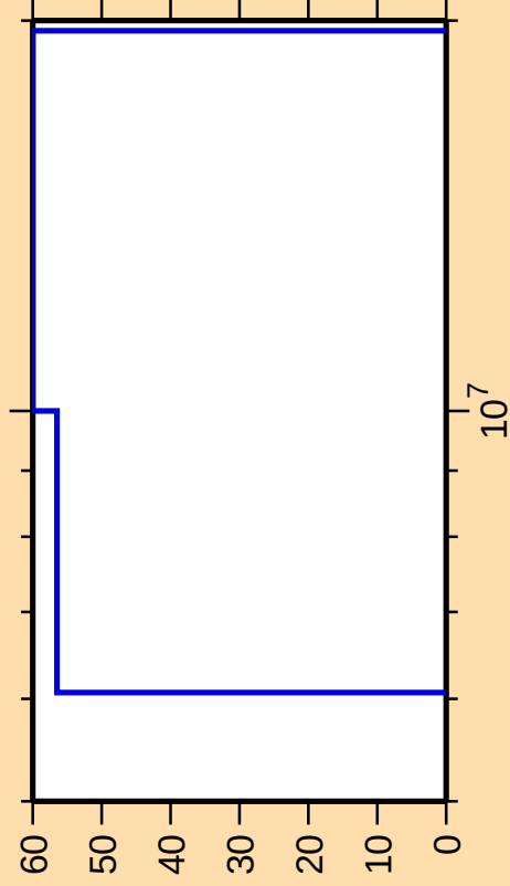
\Delta\sigma/\sigma vs. E for ^{141}\text{Cs}(n,t)
