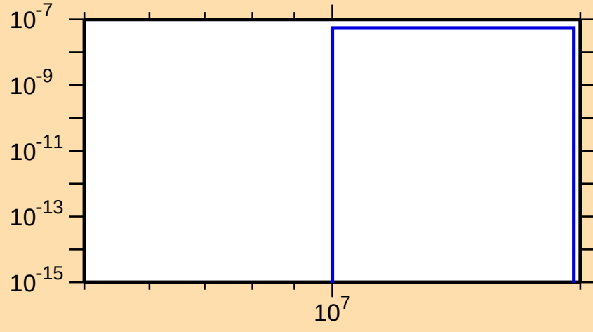
\sigma vs. E for ^{141}\text{Cs}(n,2n\alpha)
