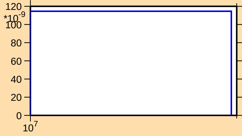
\sigma vs. E for ^{141}\text{Cs}(n,\text{nd})
