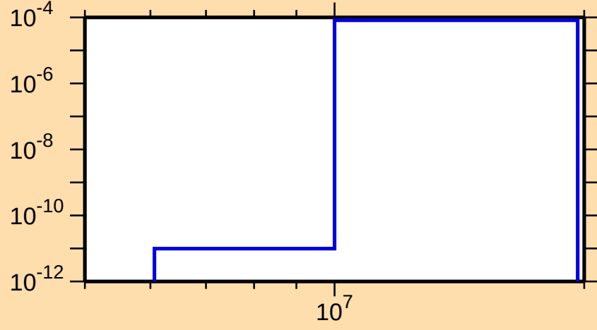
\sigma vs. E for ^{141}\text{Cs}(n,t)
