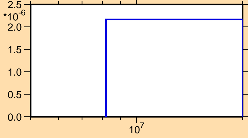
\sigma vs. E for ^{143}\text{Cs}(n,nt)
