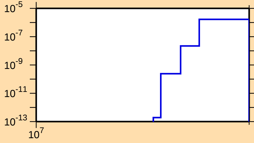
\sigma vs. E for ^{144}\text{Cs}(n,2np)
