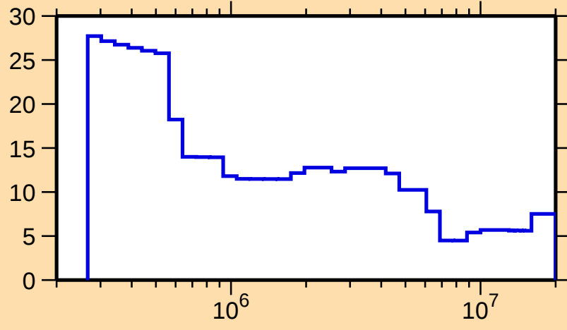
\Delta\sigma/\sigma vs. E for ^{144}\text{Cs}(n,\text{tot.})
