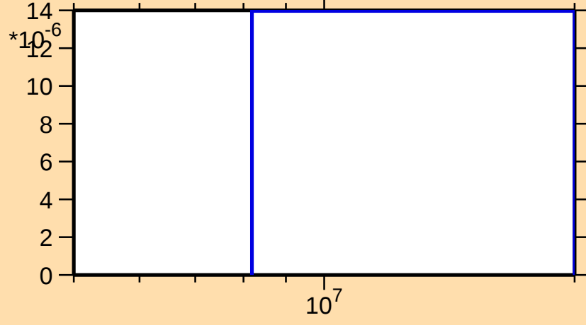
\sigma vs. E for ^{144}\text{Cs}(n,np)
