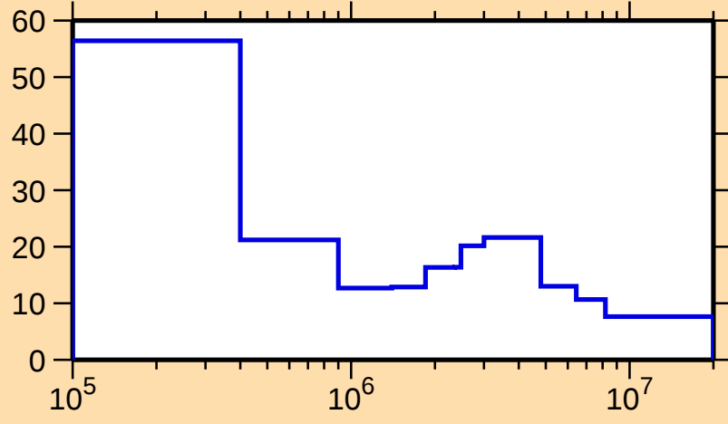
\Delta\sigma/\sigma vs. E for ^{144}\text{Cs}(n,\text{el.})
