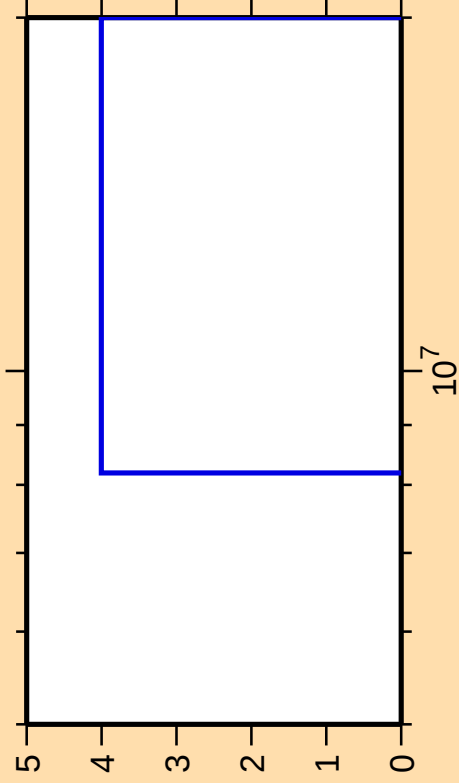
\Delta\sigma/\sigma vs. E for ^{144}\text{Cs}(n,3n)
