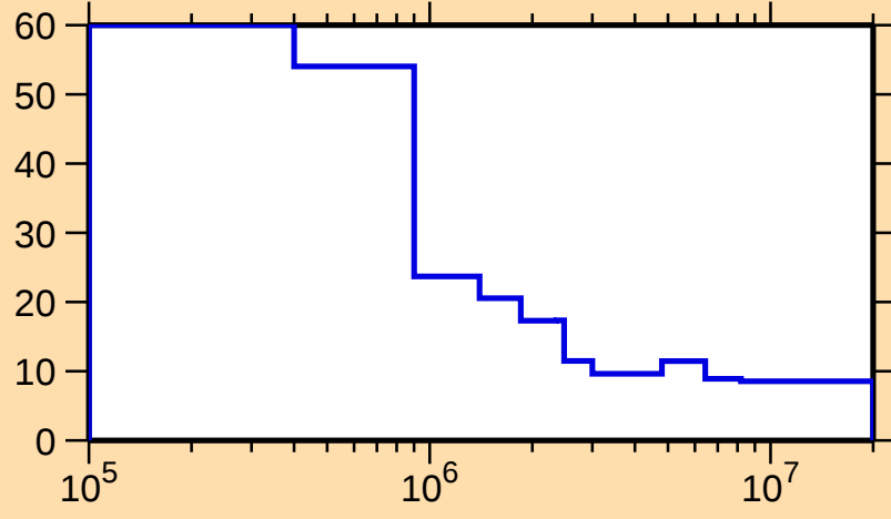
\Delta\sigma/\sigma vs. E for ^{144}\text{Cs}(n,\text{nonel.})
