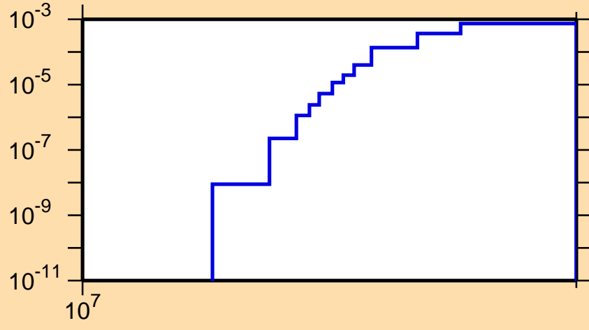
\sigma vs. E for ^{58}\text{Cu}(n,\text{nd})
