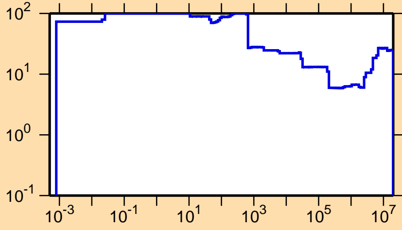
\Delta\sigma/\sigma vs. E for ^{58}\text{Cu}(n,p)
