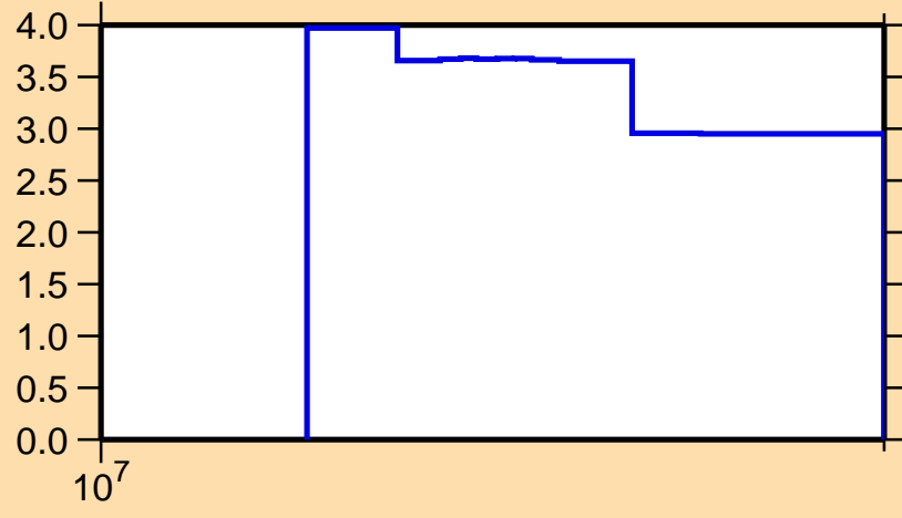
\Delta\sigma/\sigma vs. E for ^{58}\text{Cu}(n,\text{tot.})
