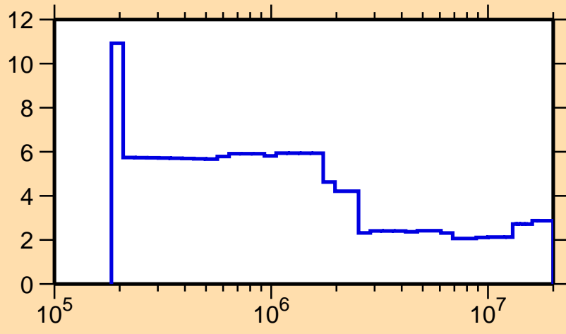
\Delta\sigma/\sigma vs. E for ^{58}\text{Cu}(n,\text{nonel.})
