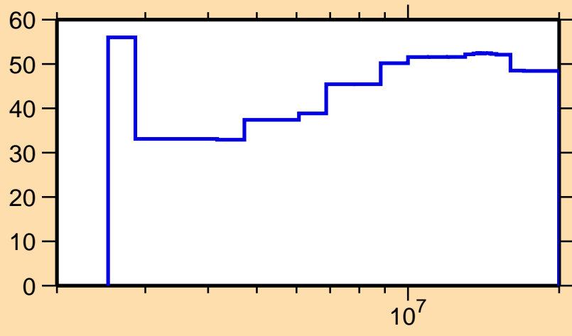
\Delta\sigma/\sigma vs. E for ^{58}\text{Cu}(n,n\text{cont.})
