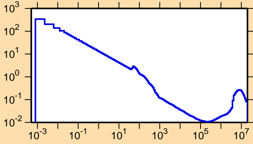
\sigma vs. E for ^{58}\text{Cu}(n,\alpha)
