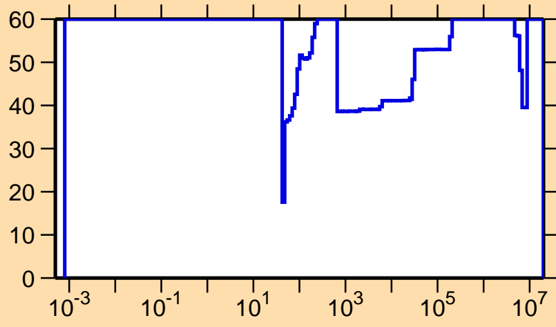
\Delta\sigma/\sigma vs. E for ^{58}\text{Cu}(n,\gamma)
