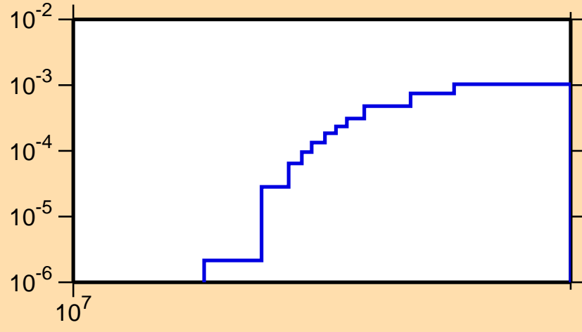
\sigma vs. E for ^{58}\text{Cu}(n,2n)
