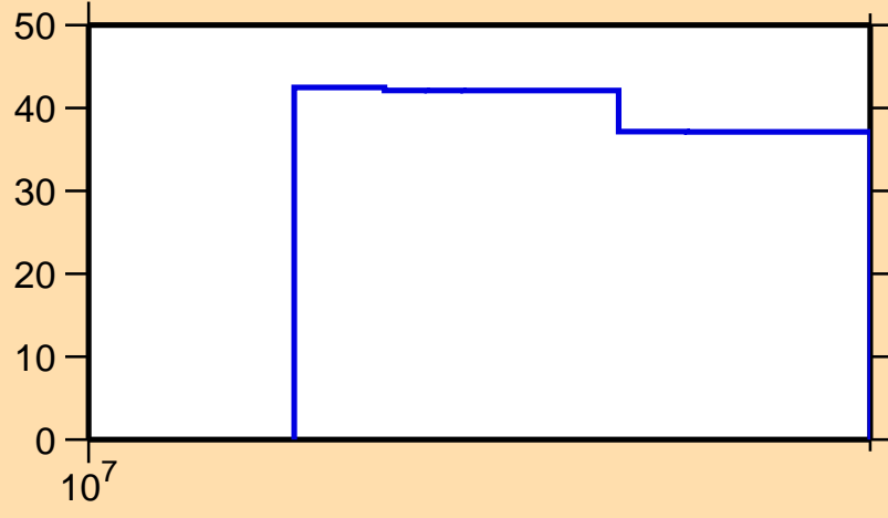
\Delta\sigma/\sigma vs. E for ^{58}\text{Cu}(n,2n)
