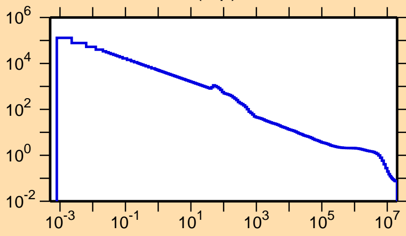
\sigma vs. E for ^{58}\text{Cu}(n,p)
