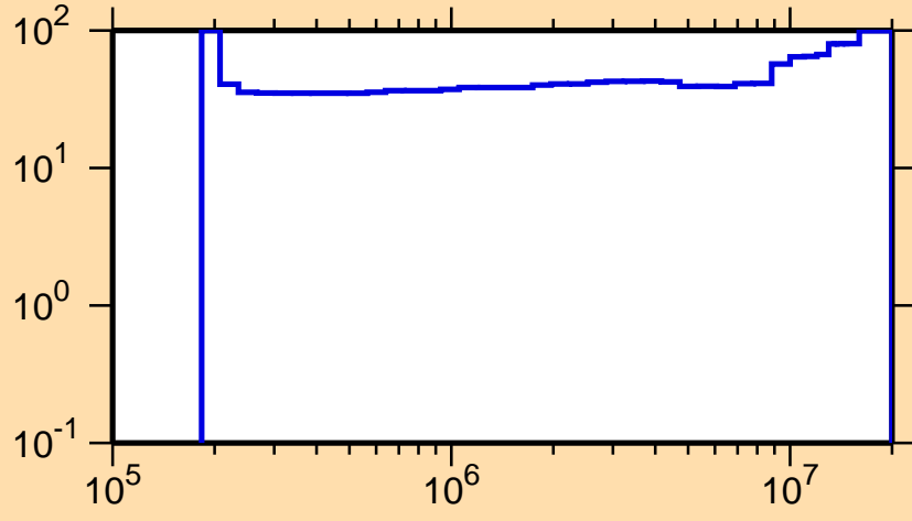
\Delta\sigma/\sigma vs. E for ^{58}\text{Cu}(n,n_1)
