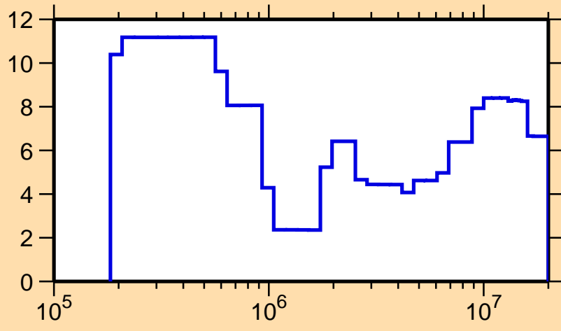
\Delta\sigma/\sigma vs. E for ^{58}\text{Cu}(n,\text{el.})
