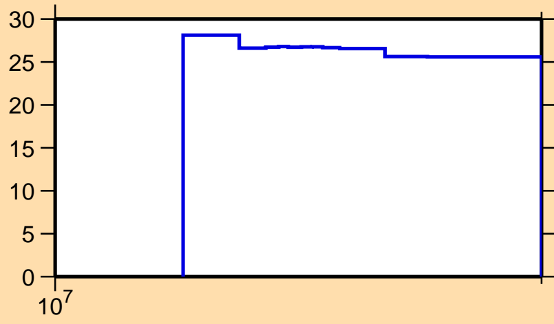
\Delta\sigma/\sigma vs. E for ^{58}\text{Cu}(n,\text{inel.})
