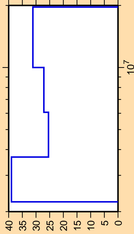
\Delta\sigma/\sigma vs. E for ^{58}\text{Cu}(n,np)
