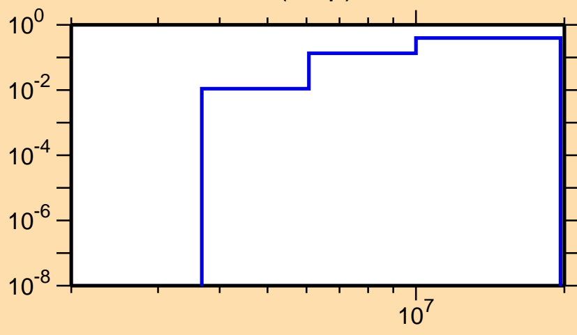
\sigma vs. E for ^{58}\text{Cu}(n,np)
