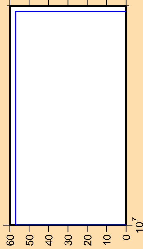
\Delta\sigma/\sigma vs. E for ^{58}\text{Cu} (mt117)
