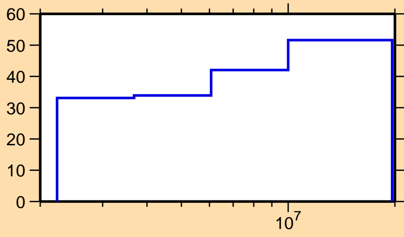
\Delta\sigma/\sigma vs. E for ^{58}\text{Cu}(n,ncont.)
