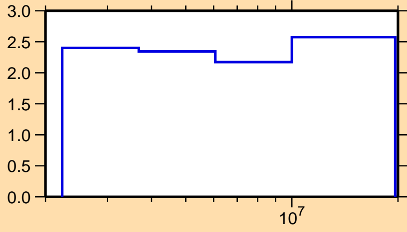
\Delta\sigma/\sigma vs. E for ^{58}\text{Cu}(n,n\text{nonel.})
