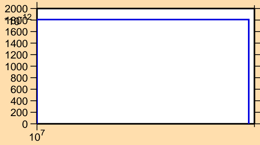
\sigma vs. E for ^{58}\text{Cu} (mt117)
