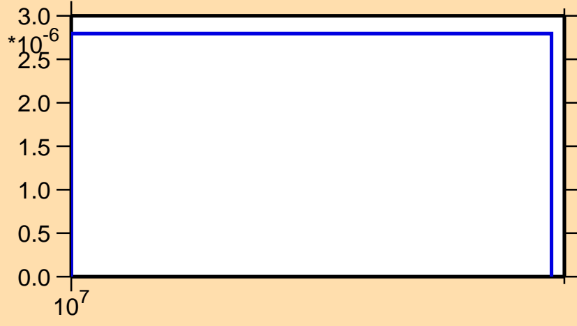
\sigma vs. E for ^{58}\text{Cu}(n,\text{pt})
