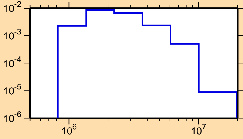
\sigma vs. E for ^{58}\text{Cu}(n,n_3)
