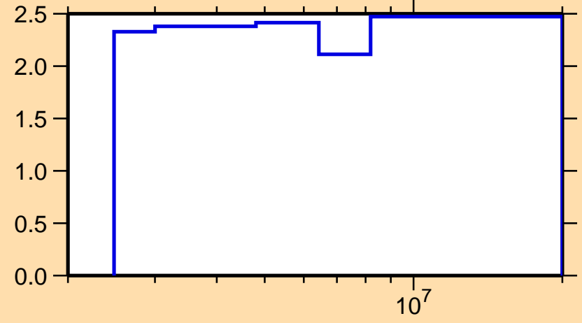
\Delta\sigma/\sigma vs. E for ^{58}\text{Cu}(n,n\text{nonel.})
