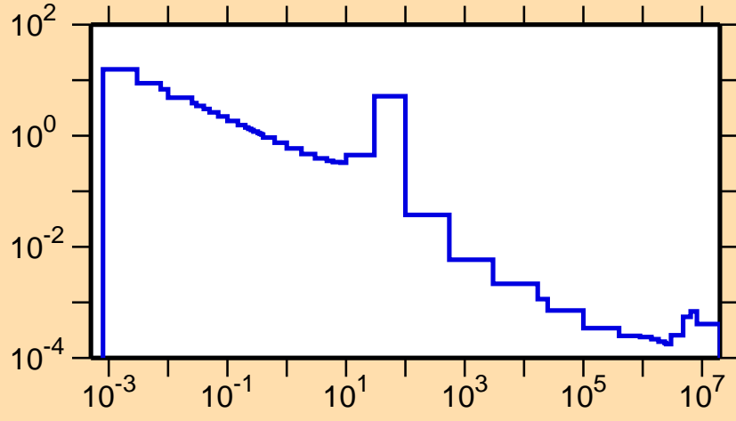
\sigma vs. E for ^{58}\text{Cu}(n,\gamma)
