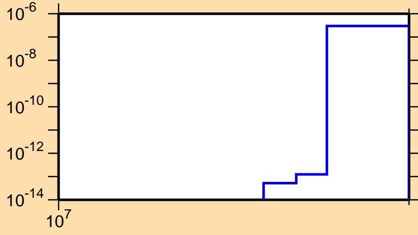
\sigma vs. E for ^{59}\text{Cu}(n,\text{pt})
