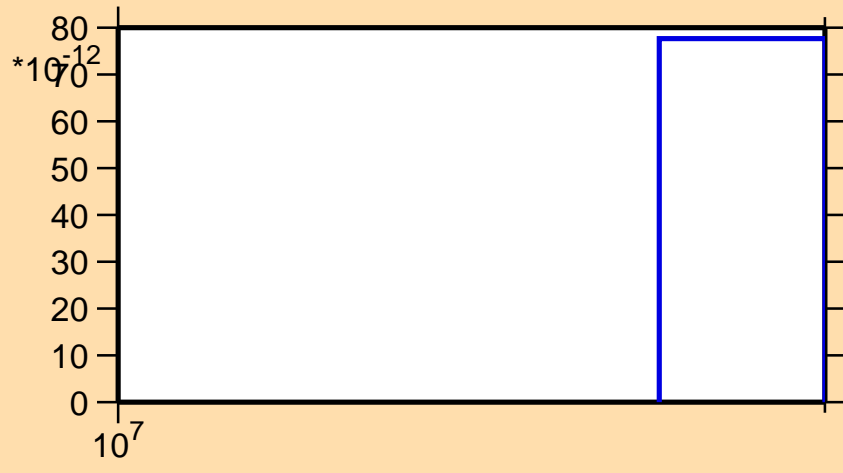
\sigma vs. E for ^{59}\text{Cu}(n,nt)
