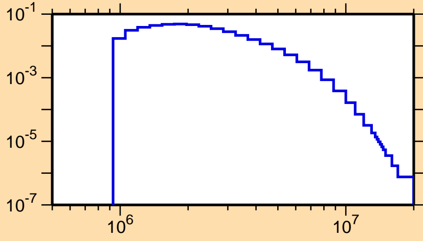
\sigma vs. E for ^{59}\text{Cu}(n,n_2)
