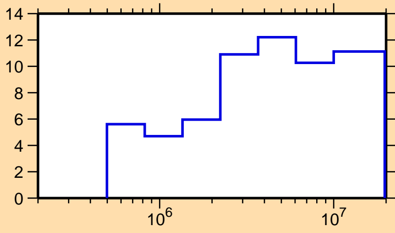
\Delta\sigma/\sigma vs. E for ^{59}\text{Cu}(n,\text{nonel.})
