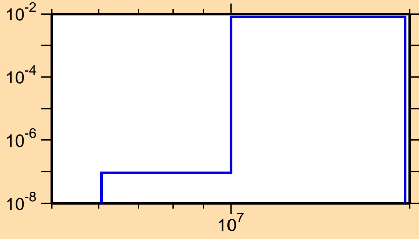
\sigma vs. E for ^{59}\text{Cu}(n,n\alpha)
