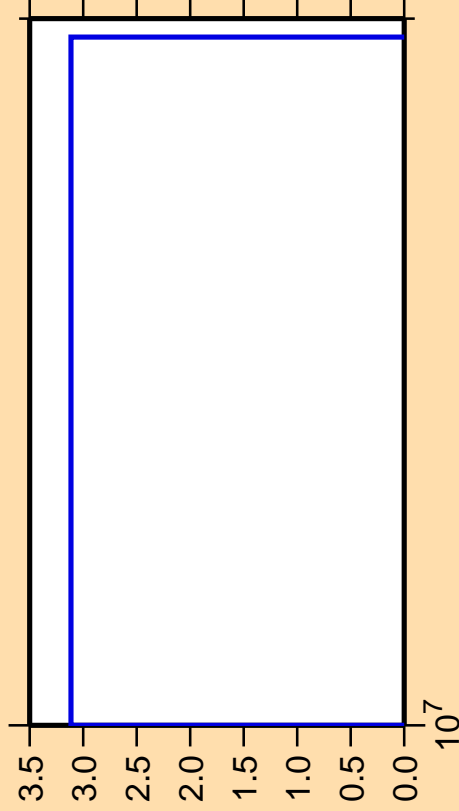
\Delta\sigma/\sigma vs. E for ^{59}\text{Cu} (mt 34)
