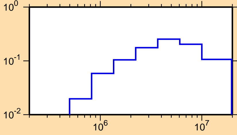
\sigma vs. E for ^{59}\text{Cu}(n,\text{inel.})
