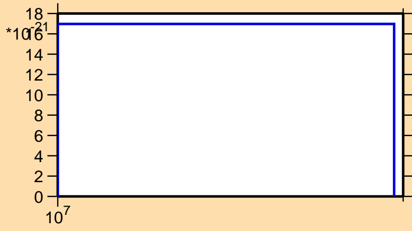
\sigma vs. E for ^{59}\text{Cu}(n,2n\alpha)
