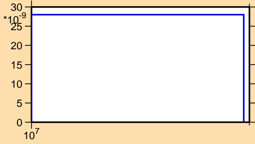
\sigma vs. E for ^{59}\text{Cu} (mt 45)
