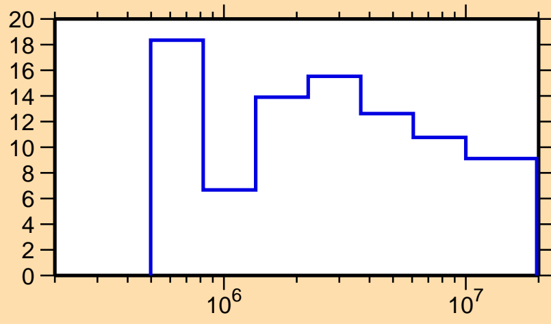
\Delta\sigma/\sigma vs. E for ^{59}\text{Cu}(n,\text{el.})
