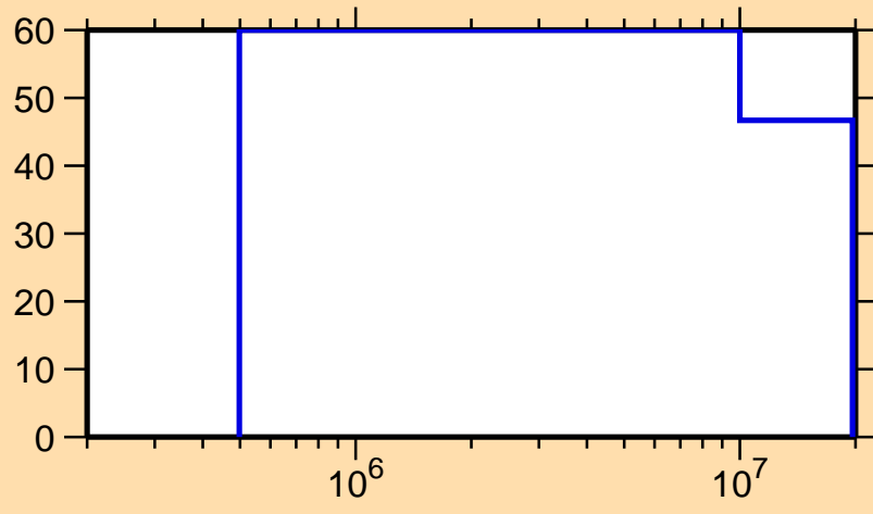
\Delta\sigma/\sigma vs. E for ^{59}\text{Cu}(n,\text{inel.})
