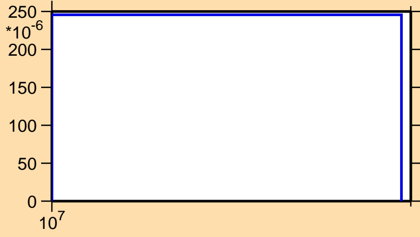
\sigma vs. E for ^{59}\text{Cu}(n,2n)
