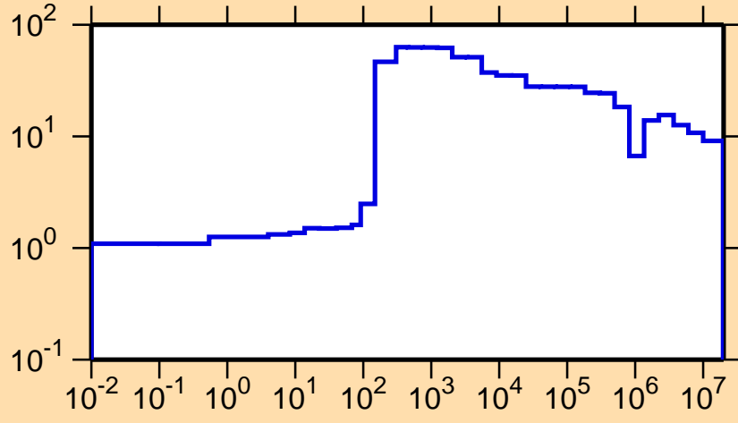
\Delta\sigma/\sigma vs. E for ^{59}\text{Cu}(n,\text{el.})
