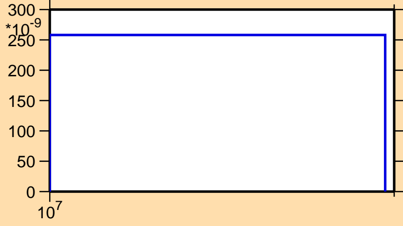
\sigma vs. E for ^{59}\text{Cu}(n,2np)
