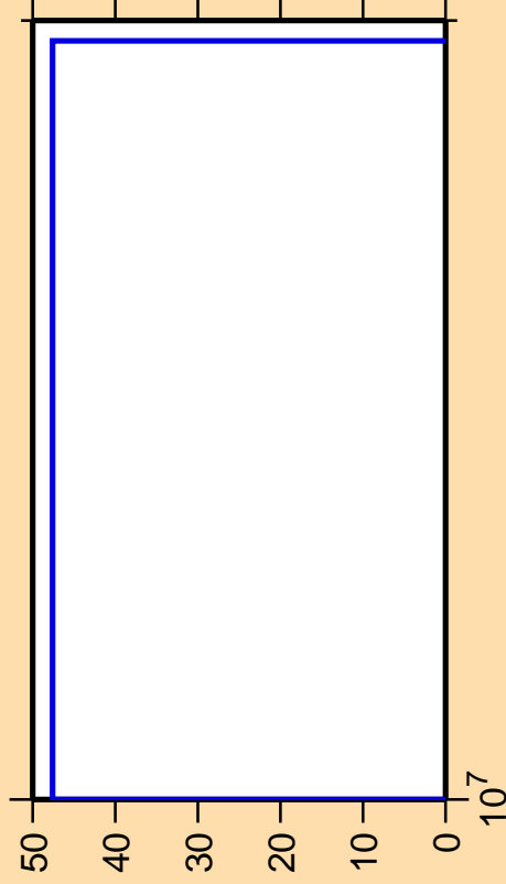
\Delta\sigma/\sigma vs. E for ^{59}\text{Cu}(n,n\text{cont.})
