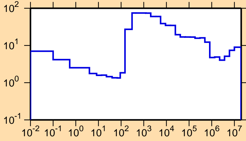
\Delta\sigma/\sigma vs. E for ^{59}\text{Cu}(n,\text{tot.})
