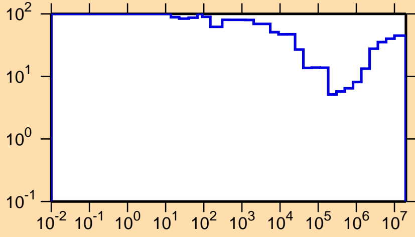
\Delta\sigma/\sigma vs. E for ^{59}\text{Cu}(n,p)
