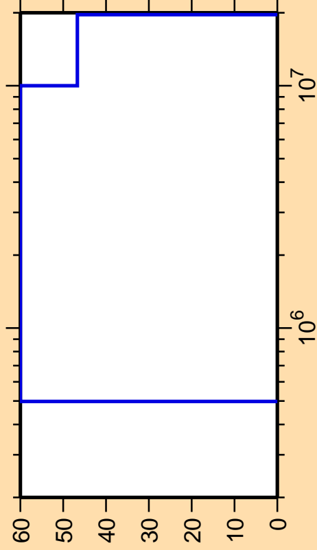
\Delta\sigma/\sigma vs. E for ^{59}\text{Cu}(n,\text{inel.})
