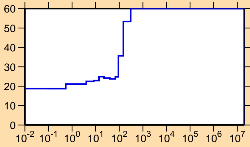
\Delta\sigma/\sigma vs. E for ^{59}\text{Cu}(n,\gamma)
