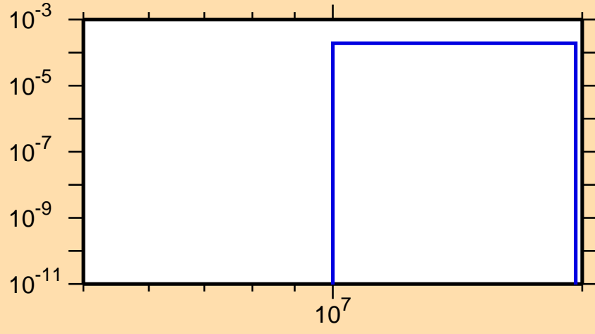
\sigma vs. E for ^{59}\text{Cu}(n,\text{pd})
