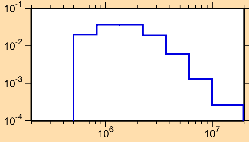
\sigma vs. E for ^{59}\text{Cu}(n,n_1)
