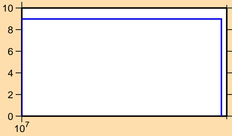
\Delta\sigma/\sigma vs. E for ^{59}\text{Cu}(n,\text{tot.})
