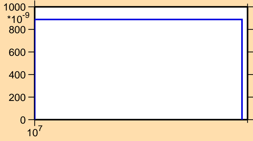
\sigma vs. E for ^{59}\text{Cu}(n,\text{nd})
