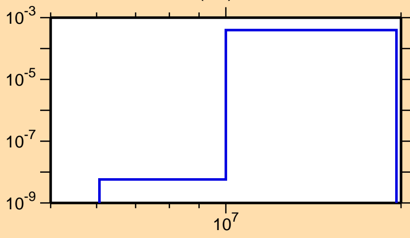
\sigma vs. E for ^{59}\text{Cu}(n,t)
