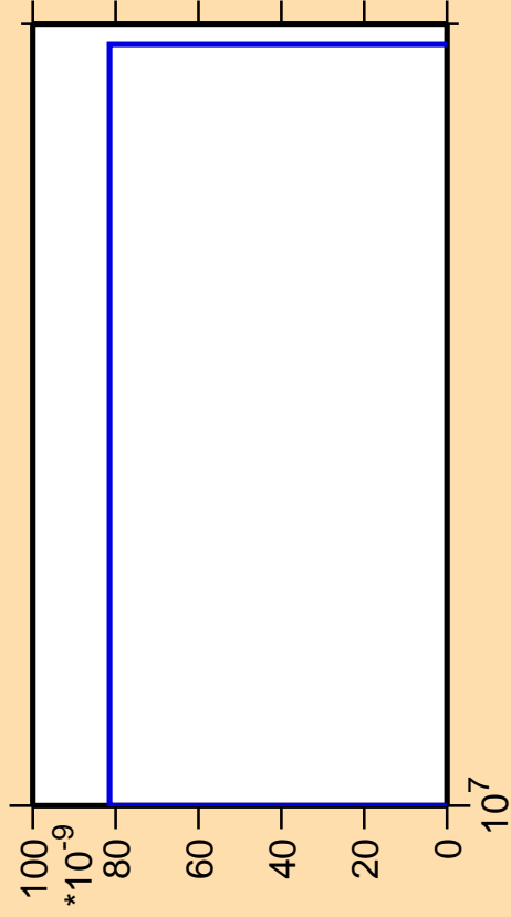
\Delta\sigma/\sigma vs. E for ^{59}\text{Cu}(n,2n\alpha)
