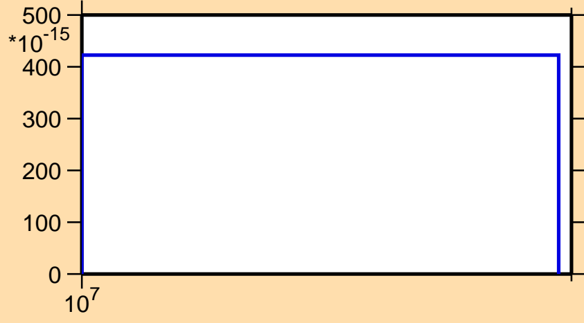
\sigma vs. E for ^{59}\text{Cu}(n,nt)
