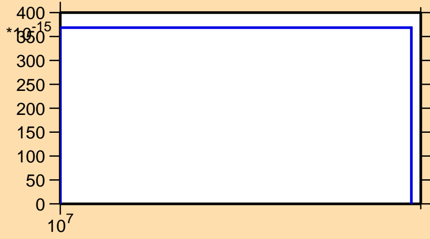
\sigma vs. E for ^{59}\text{Cu} (mt 34)
