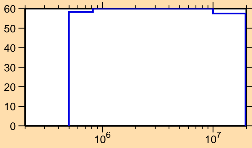
\Delta\sigma/\sigma vs. E for ^{59}\text{Cu}(n,n_1)
