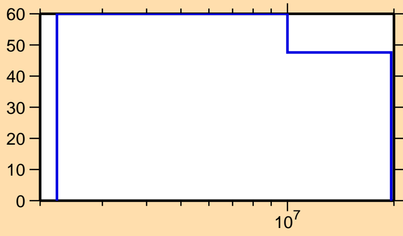
\Delta\sigma/\sigma vs. E for ^{59}\text{Cu}(n,n\text{cont.})
