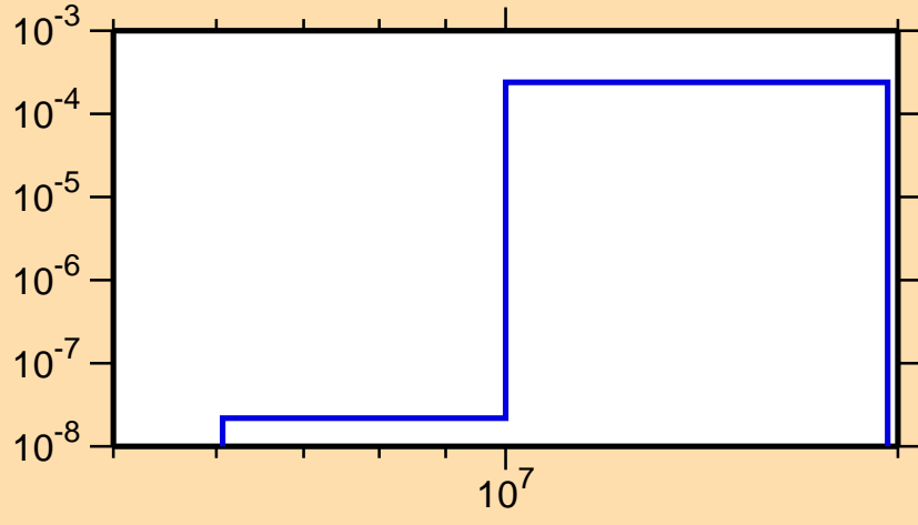
\sigma vs. E for ^{59}\text{Cu}(n,\text{He3})
