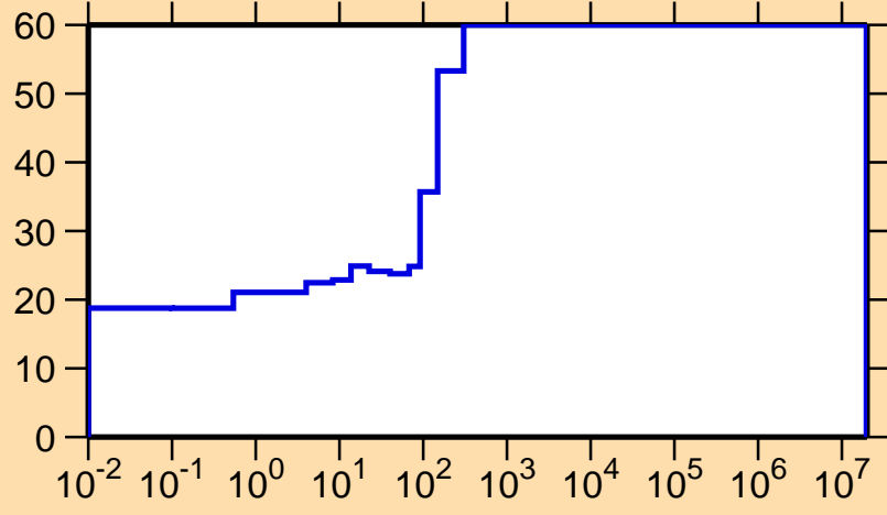
\Delta\sigma/\sigma vs. E for ^{59}\text{Cu}(n,\gamma)
