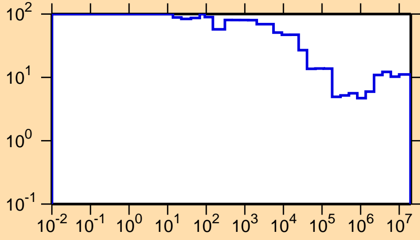
\Delta\sigma/\sigma vs. E for ^{59}\text{Cu}(n,\text{nonel.})
