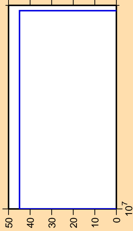
\Delta\sigma/\sigma vs. E for ^{59}\text{Cu}(n,p)
