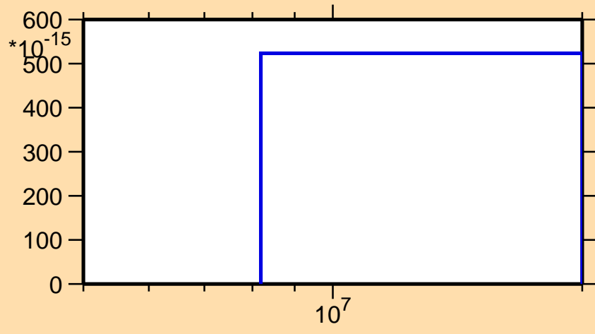
\sigma vs. E for ^{59}\text{Cu} (mt 34)
