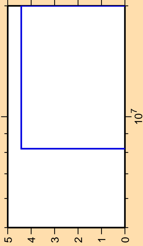
\Delta\sigma/\sigma vs. E for ^{59}\text{Cu} (mt 34)
