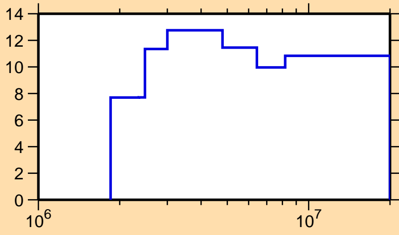
\Delta\sigma/\sigma vs. E for ^{59}\text{Cu}(n,n\text{nonel.})
