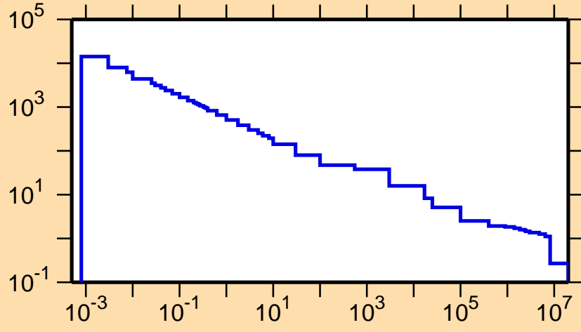
\sigma vs. E for ^{59}\text{Cu}(n,p)
