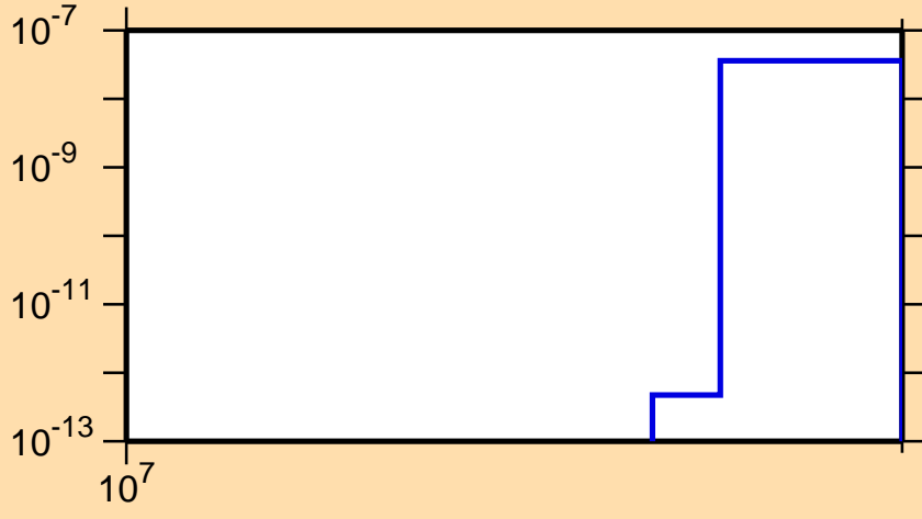
\sigma vs. E for ^{60}\text{Cu} (mt 34)
