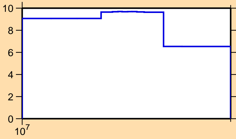
\Delta\sigma/\sigma vs. E for ^{60}\text{Cu}(n,\text{tot.})
