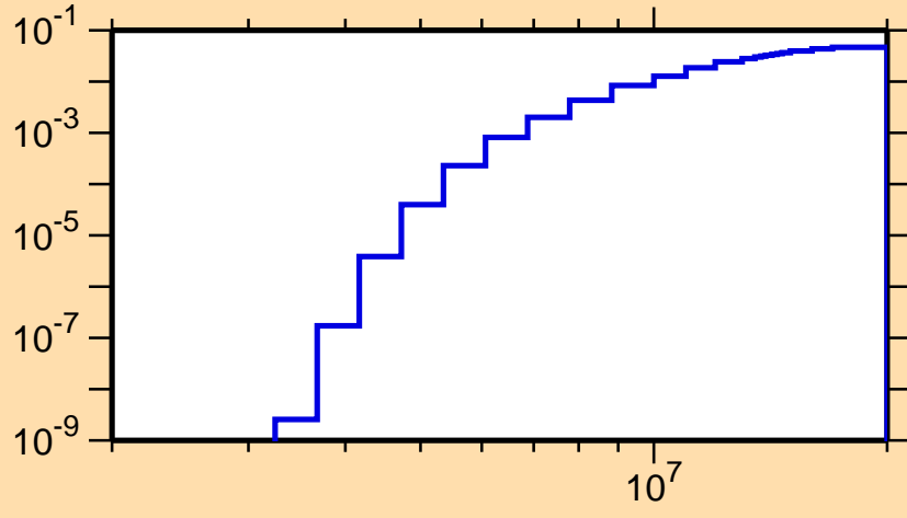
\sigma vs. E for ^{60}\text{Cu}(n,d)
