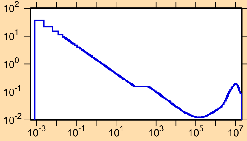
\sigma vs. E for ^{60}\text{Cu}(n,\alpha)
