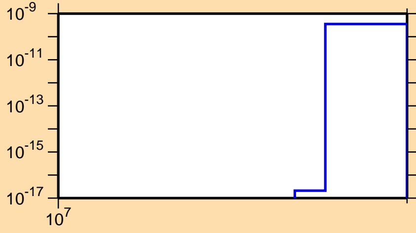
\sigma vs. E for ^{60}\text{Cu}(n,2n\alpha)
