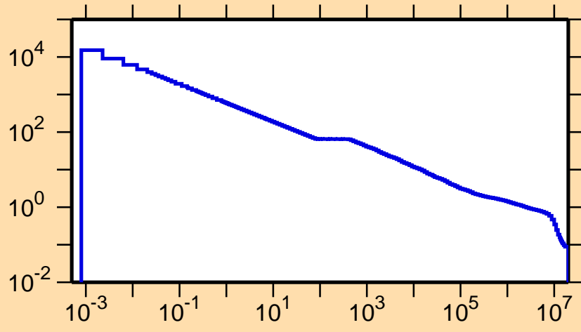
\sigma vs. E for ^{60}\text{Cu}(n,p)
