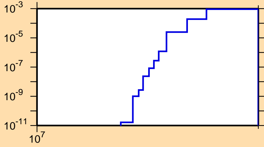
\sigma vs. E for ^{60}\text{Cu}(n,\text{pd})
