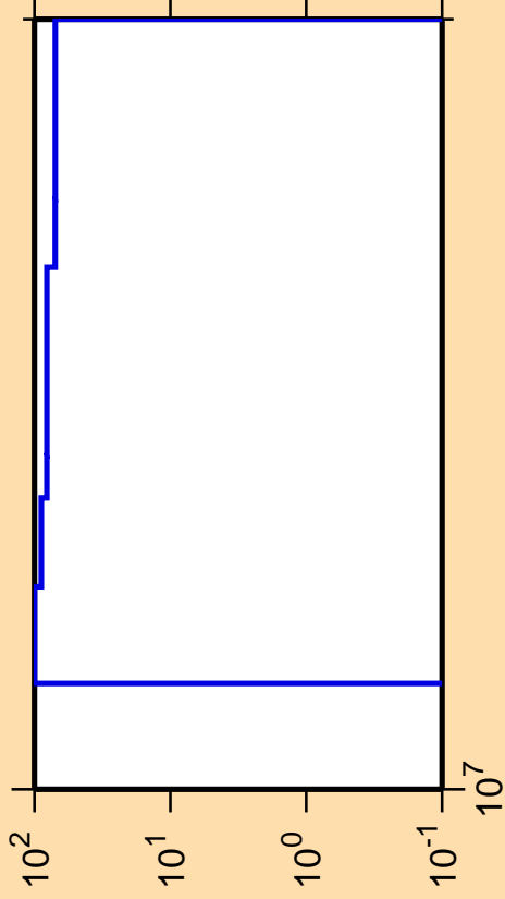
\Delta\sigma/\sigma vs. E for ^{60}\text{Cu}(n,nd)
