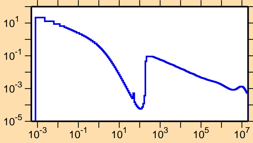
\sigma vs. E for ^{60}\text{Cu}(n,\gamma)
