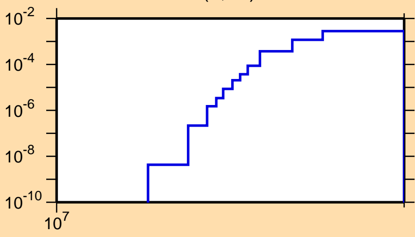
\sigma vs. E for ^{60}\text{Cu}(n,nd)
