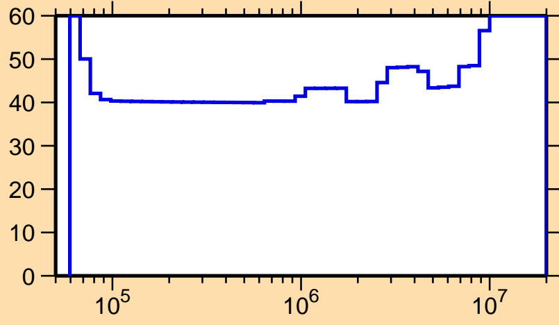
\Delta\sigma/\sigma vs. E for ^{60}\text{Cu}(n,n_1)
