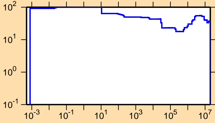
\Delta\sigma/\sigma vs. E for ^{60}\text{Cu}(n,p)
