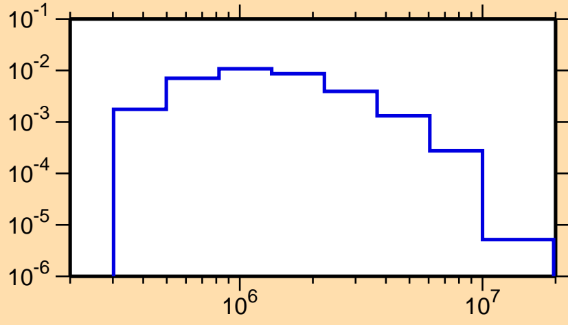
\sigma vs. E for ^{60}\text{Cu}(n,n_3)
