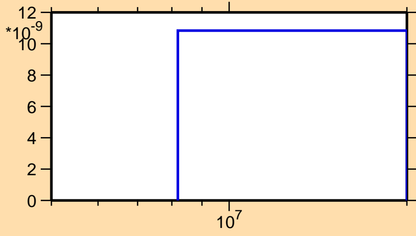
\sigma vs. E for ^{60}\text{Cu}(\text{mt } 45)
