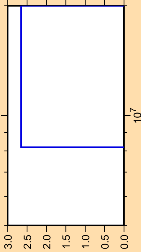
\Delta\sigma/\sigma vs. E for ^{60}\text{Cu}(n,nt)
