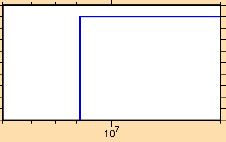
\sigma vs. E for ^{60}\text{Cu}(n,\text{pd})
