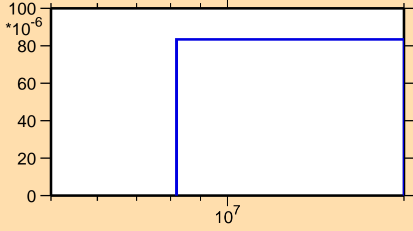
\sigma vs. E for ^{60}\text{Cu}(n,2np)
