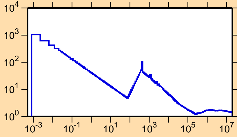
\sigma vs. E for ^{62}\text{Cu}(n,\text{nonel.})
