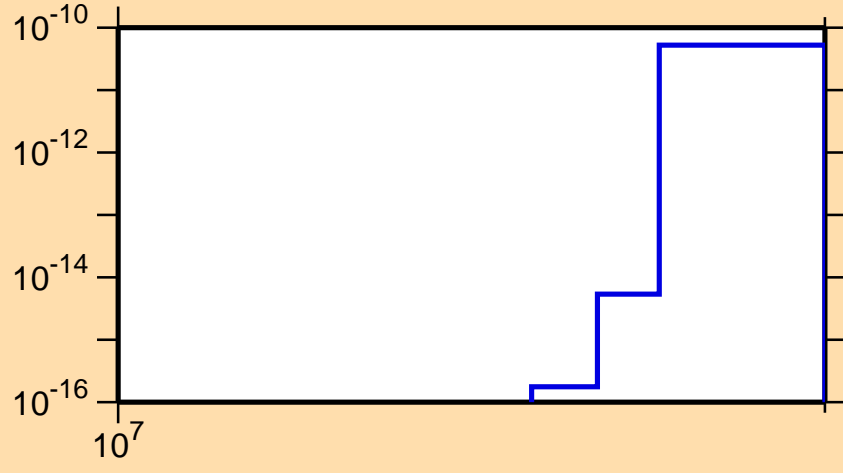
\sigma vs. E for ^{62}\text{Cu} (mt 34)
