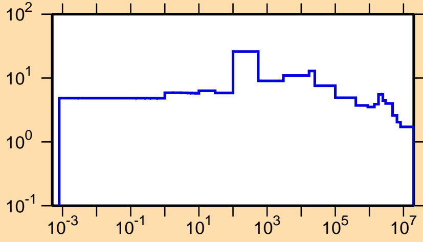
\Delta\sigma/\sigma vs. E for ^{62}\text{Cu}(n,el.)
