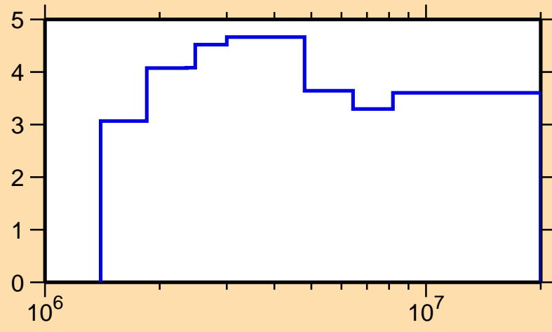
\Delta\sigma/\sigma vs. E for ^{62}\text{Cu}(n,n\text{onel.})
