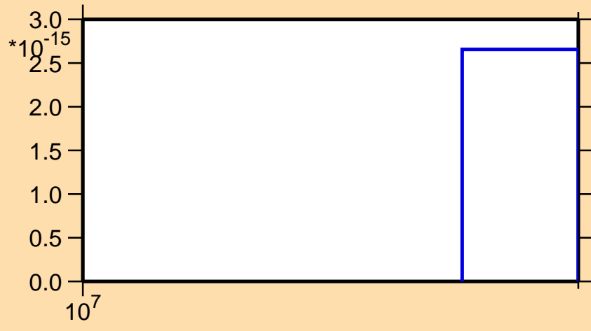
\sigma vs. E for ^{63}\text{Cu} (mt 34)
