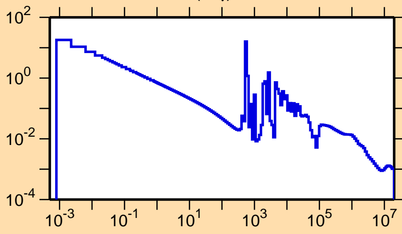
\sigma vs. E for ^{63}\text{Cu}(n,\gamma)
