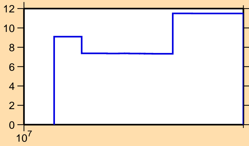
\Delta\sigma/\sigma vs. E for ^{63}\text{Cu}(n,2n)
