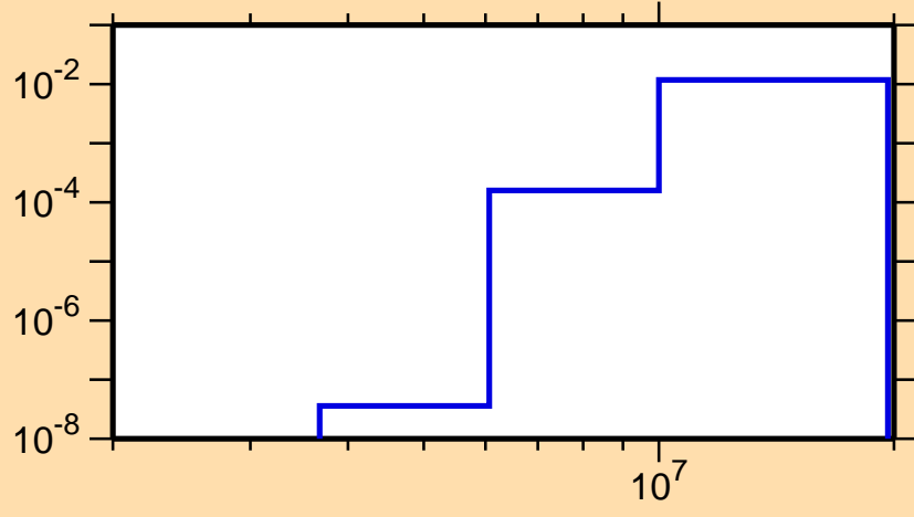
\sigma vs. E for ^{63}\text{Cu}(n,d)
