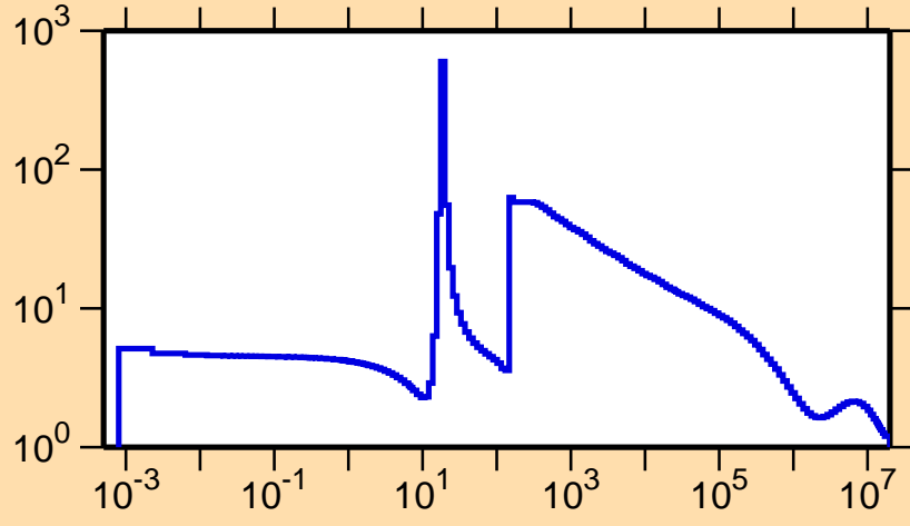
\sigma vs. E for ^{64}\text{Cu}(n,\text{el.})
