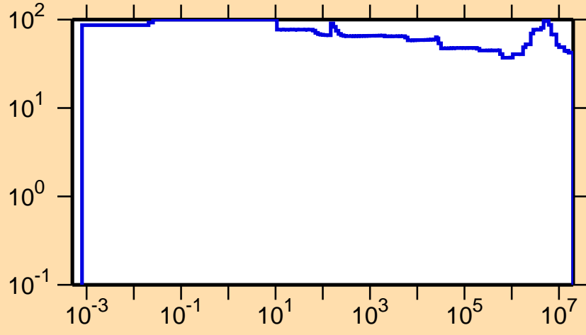
\Delta\sigma/\sigma vs. E for ^{64}\text{Cu}(n,p)
