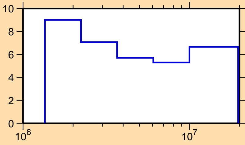
\Delta\sigma/\sigma vs. E for ^{64}\text{Cu}(n,n\text{nonel.})
