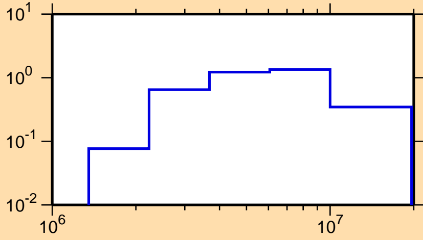
\sigma vs. E for ^{64}\text{Cu}(n,n\text{cont.})
