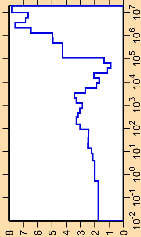
\Delta\sigma/\sigma vs. E for ^{65}\text{Cu}(n,\text{el.})
