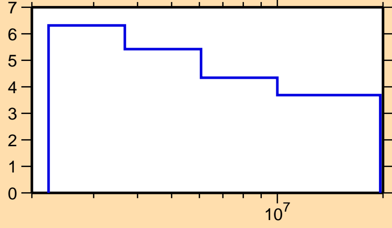
\Delta\sigma/\sigma vs. E for ^{65}\text{Cu}(n,n\text{onel.})
