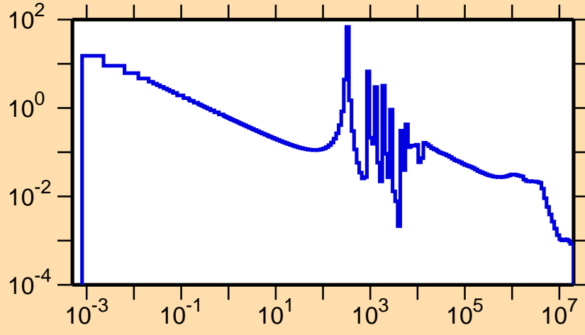
\sigma vs. E for ^{67}\text{Cu}(n,\gamma)
