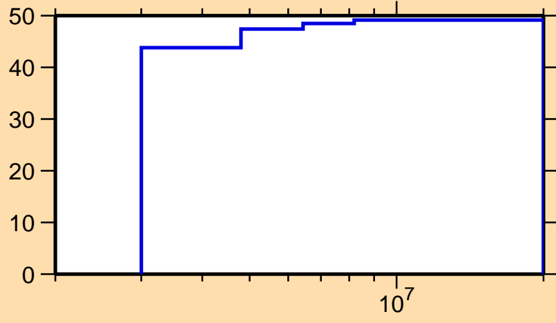
\Delta\sigma/\sigma vs. E for ^{67}\text{Cu}(n,p)
