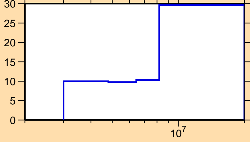
\Delta\sigma/\sigma vs. E for ^{67}\text{Cu}(n,n\text{cont.})
