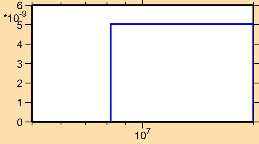
\sigma vs. E for ^{67}\text{Cu}(n,nt)
