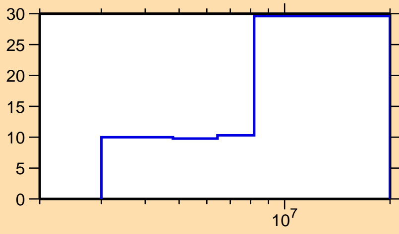
\Delta\sigma/\sigma vs. E for ^{67}\text{Cu}(n,n\text{cont.})
