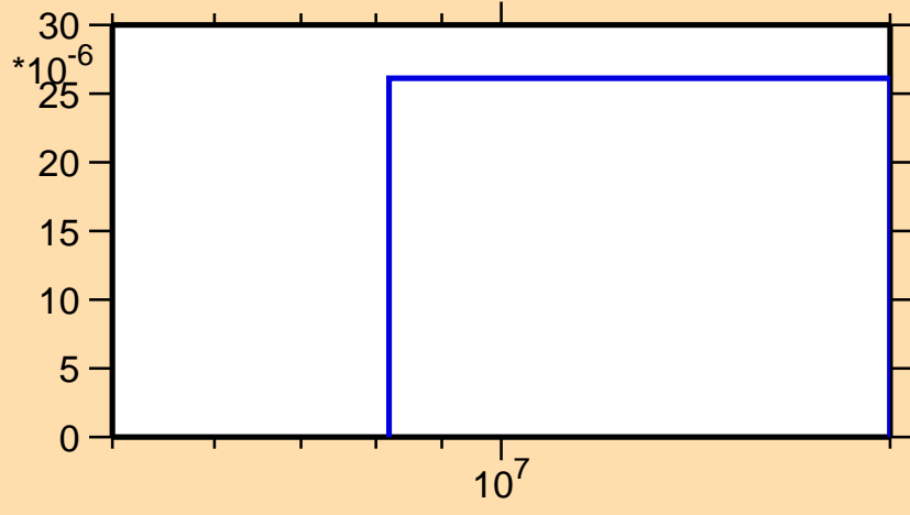
\sigma vs. E for ^{67}\text{Cu}(n,t)
