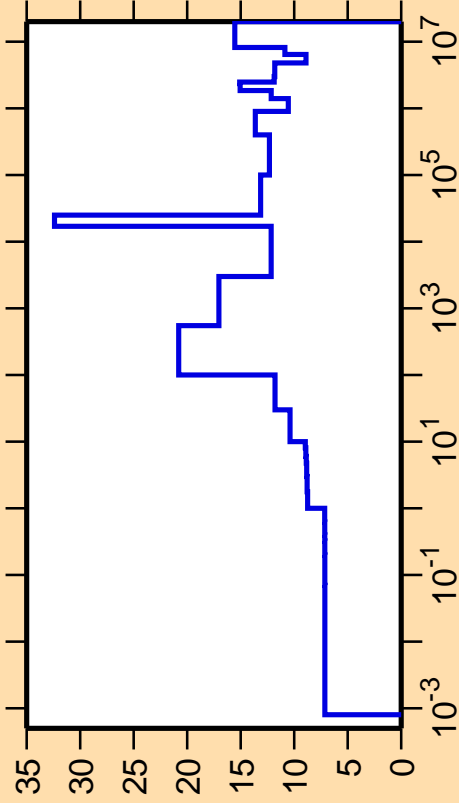
\Delta\sigma/\sigma vs. E for ^{67}\text{Cu}(n,\text{el.})
