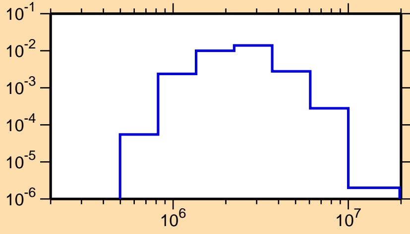
\sigma vs. E for ^{68}\text{Cu}(n,n_3)
