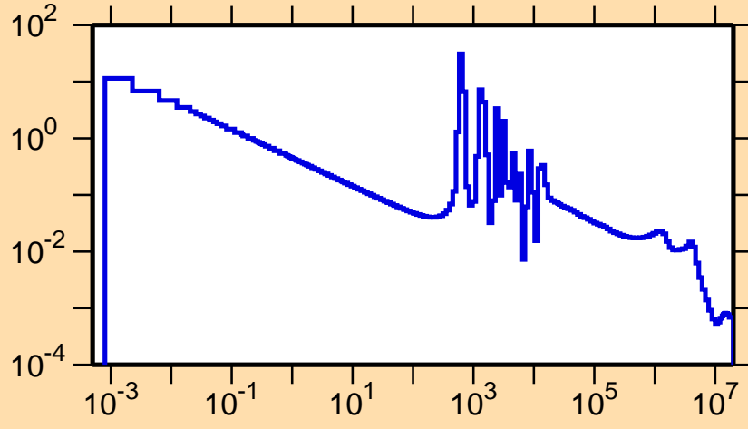
\sigma vs. E for ^{69}\text{Cu}(n,\gamma)
