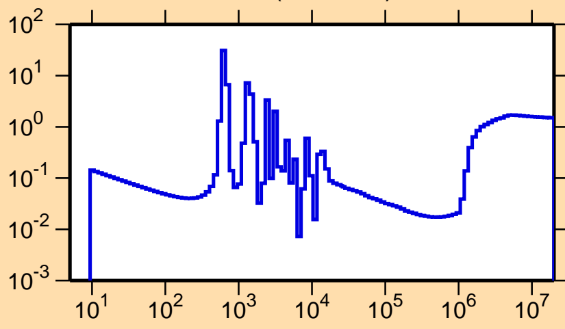
\sigma vs. E for ^{69}\text{Cu}(n,\text{nonel.})
