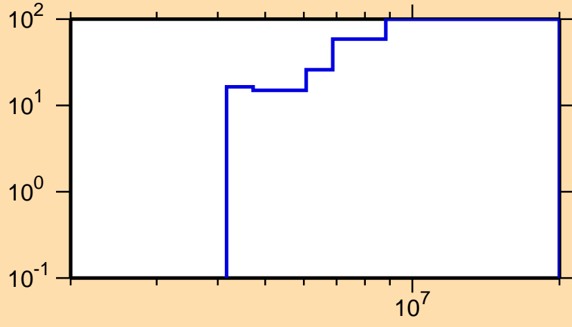
\Delta\sigma/\sigma vs. E for ^{70}\text{Cu}(n,n\text{cont.})
