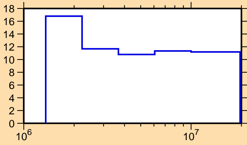
\Delta\sigma/\sigma vs. E for ^{70}\text{Cu}(n,n\text{nonel.})
