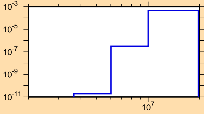
\sigma vs. E for ^{70}\text{Cu}(n,\alpha)
