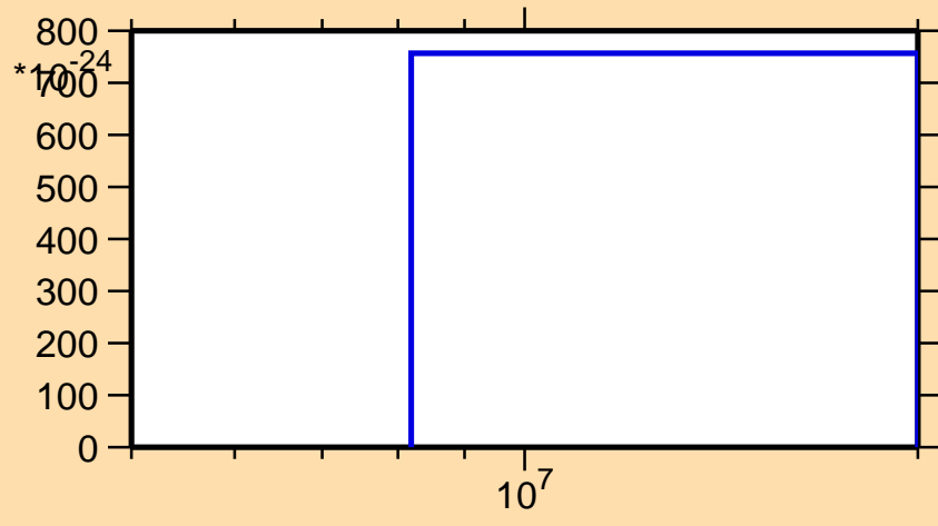
\sigma vs. E for ^{70}\text{Cu}(n,\text{He}3)
