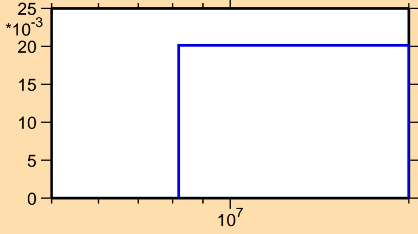
\sigma vs. E for ^{70}\text{Cu}(n,3n)
