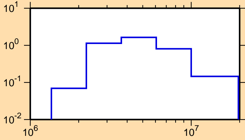
\sigma vs. E for ^{70}\text{Cu}(n,n\text{cont.})
