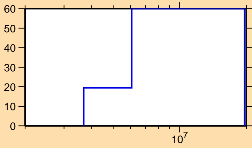
\Delta\sigma/\sigma vs. E for ^{70}\text{Cu}(n,ncont.)
