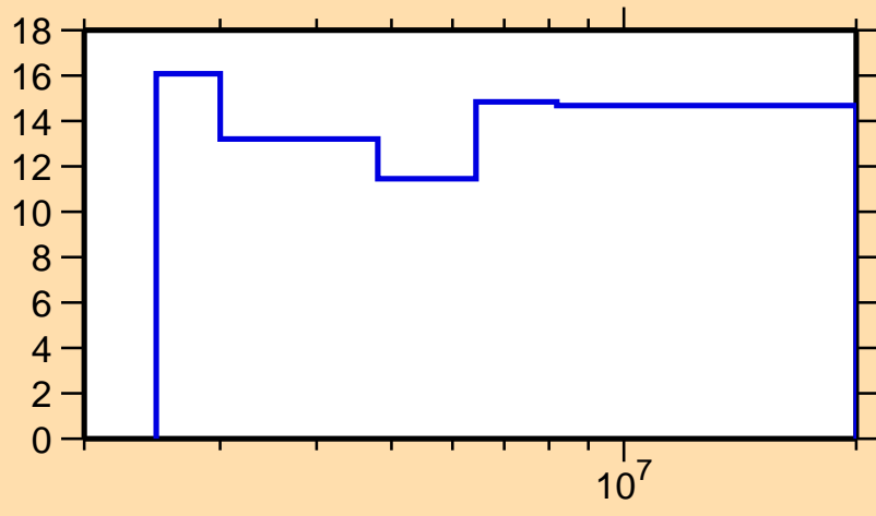
\Delta\sigma/\sigma vs. E for ^{70}\text{Cu}(n,el.)
