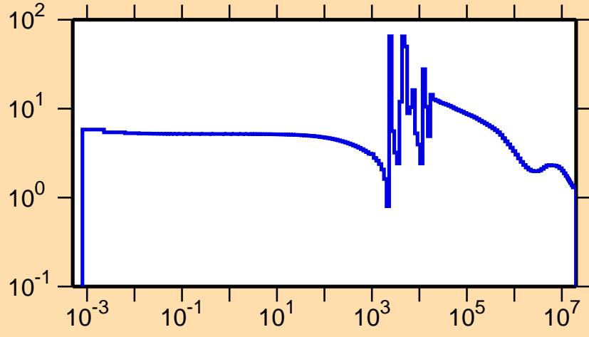
\sigma vs. E for ^{71}\text{Cu}(n,\text{el.})
