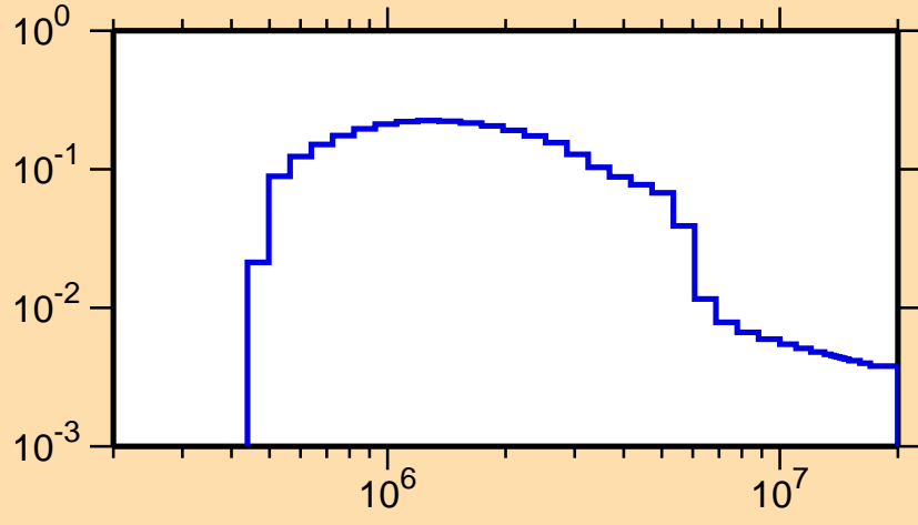
\sigma vs. E for ^{71}\text{Cu}(n,n_1)
