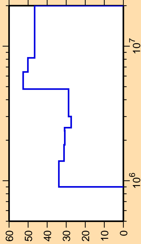
\Delta\sigma/\sigma vs. E for ^{71}\text{Cu}(n,n_4)
