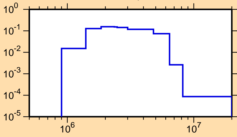
\sigma vs. E for ^{71}\text{Cu}(n,n_4)
