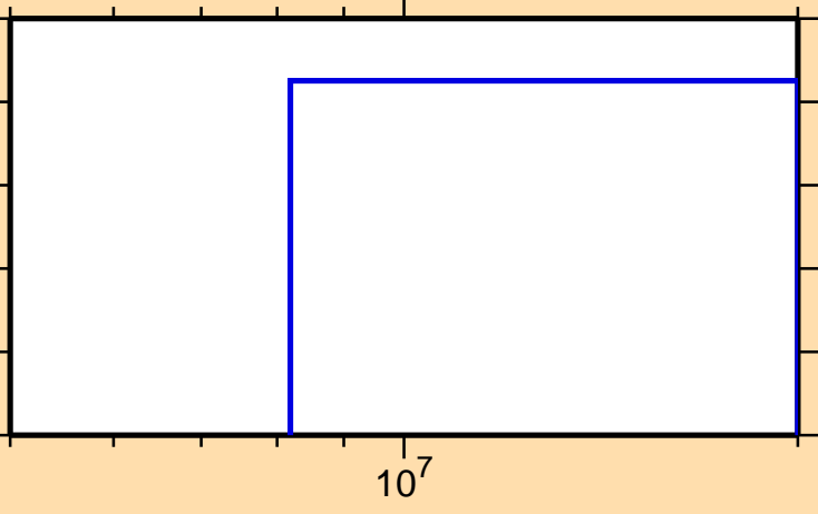
\sigma vs. E for ^{71}\text{Cu}(n,\text{nd})
