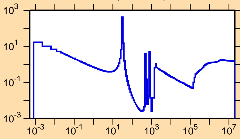
\sigma vs. E for ^{72}\text{Cu}(n,\text{nonel.})
