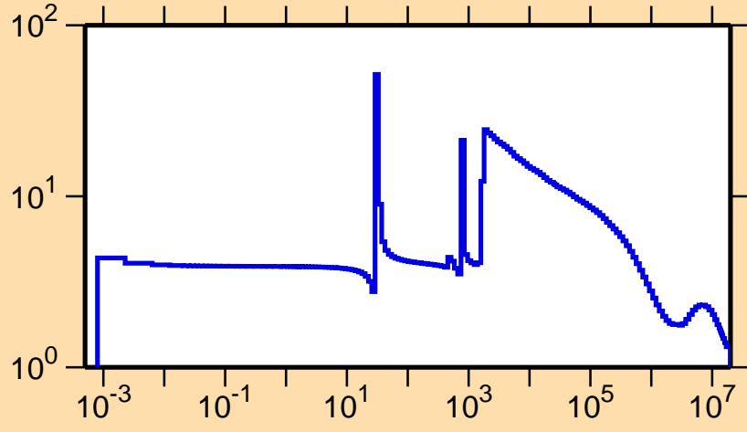
\sigma vs. E for ^{72}\text{Cu}(n,\text{el.})
