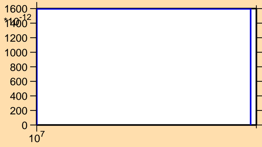
\sigma vs. E for ^{72}\text{Cu}(n,2np)
