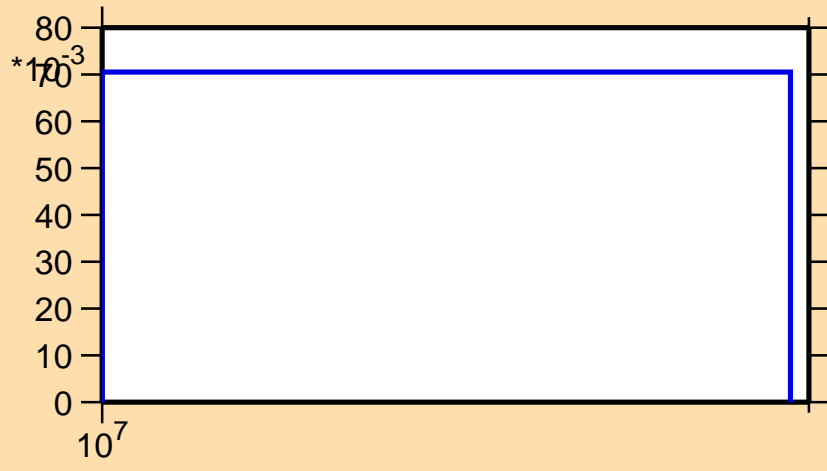
\sigma vs. E for ^{72}\text{Cu}(n,3n)
