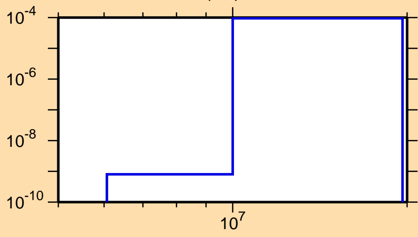
\sigma vs. E for ^{72}\text{Cu}(n,t)
