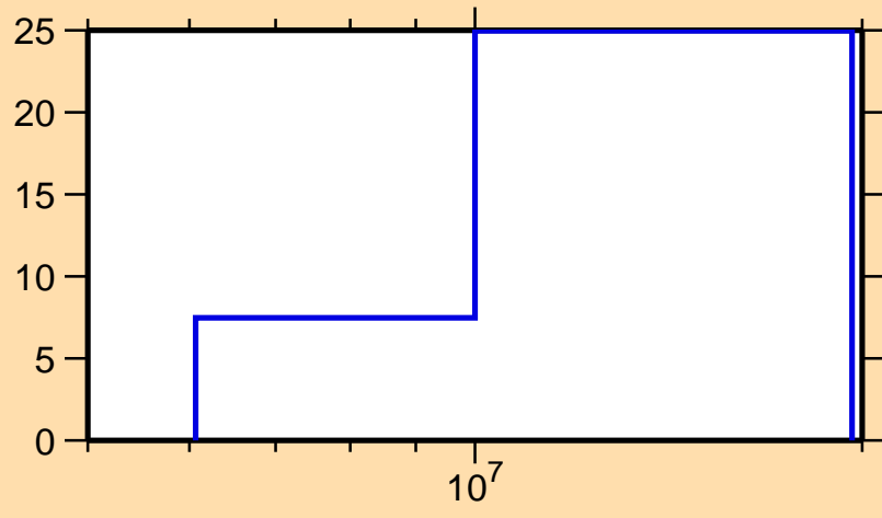
\Delta\sigma/\sigma vs. E for ^{72}\text{Cu}(n,\text{tot.})
