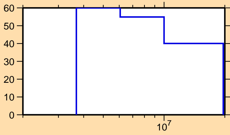
\Delta\sigma/\sigma vs. E for ^{72}\text{Cu}(n,2n)
