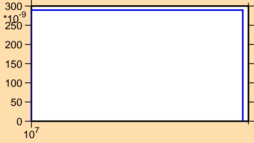
\sigma vs. E for ^{72}\text{Cu}(n,n\alpha)
