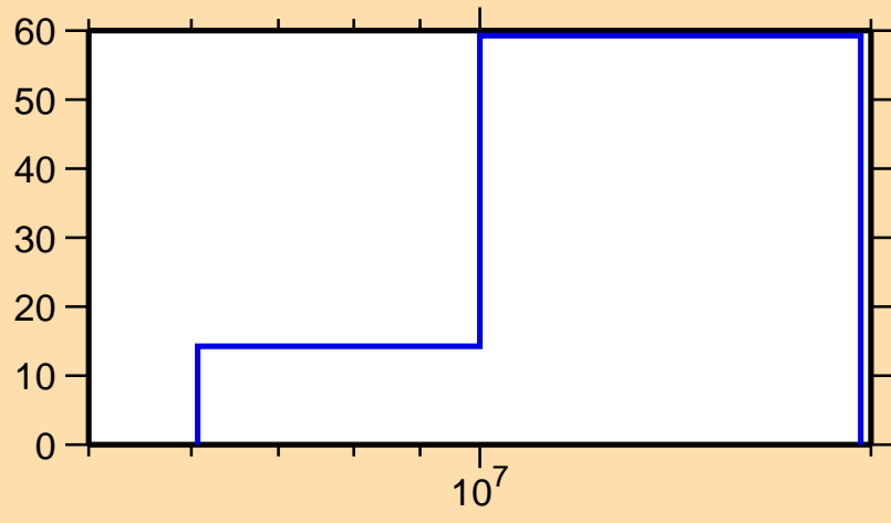
\Delta\sigma/\sigma vs. E for ^{72}\text{Cu}(n,\text{el.})
