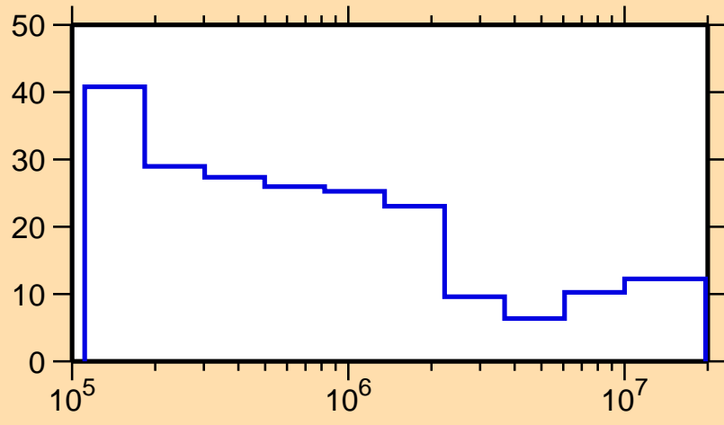
\Delta\sigma/\sigma vs. E for ^{72}\text{Cu}(n,\text{nonel.})
