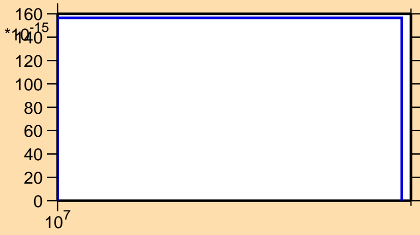
\sigma vs. E for ^{72}\text{Cu}(n,2n\alpha)
