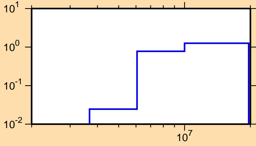
\sigma vs. E for ^{72}\text{Cu}(n,2n)
