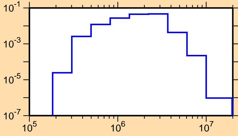
\sigma vs. E for ^{72}\text{Cu}(n,n_3)
