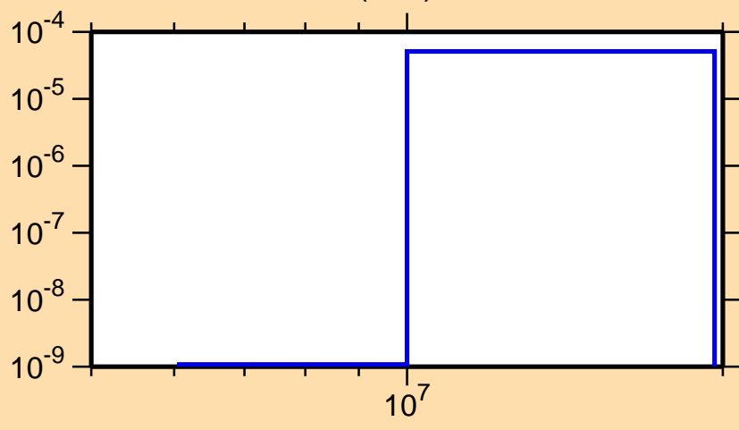
\sigma vs. E for ^{72}\text{Cu}(n,\alpha)
