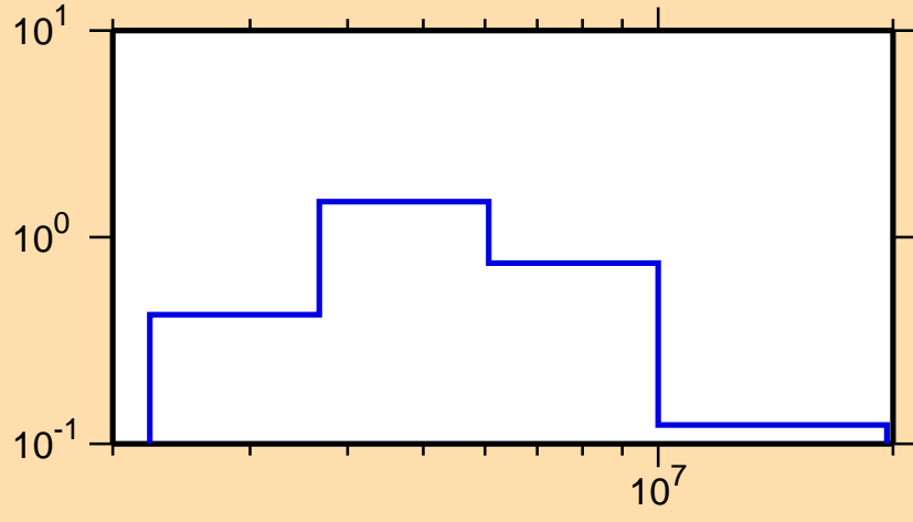
\sigma vs. E for ^{72}\text{Cu}(n,n\text{cont.})
