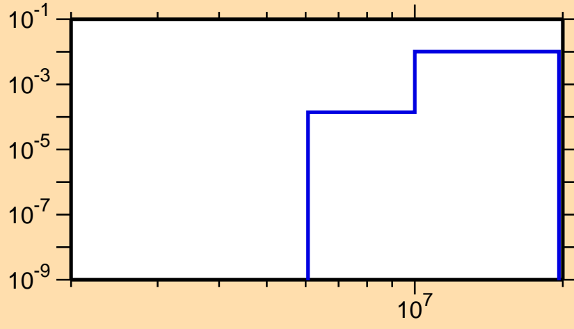
\sigma vs. E for ^{72}\text{Cu}(n,p)
