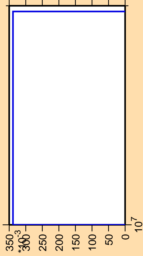
\Delta\sigma/\sigma vs. E for ^{72}\text{Cu}(n,2n\alpha)
