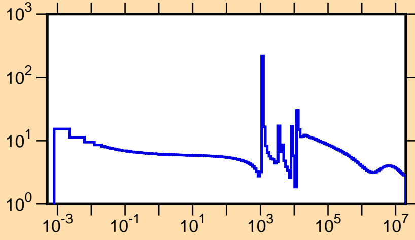
\sigma vs. E for ^{73}\text{Cu}(n,\text{tot.})
