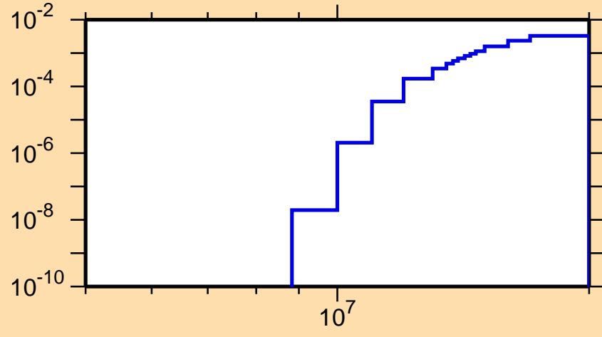
\sigma vs. E for ^{73}\text{Cu}(n,p)
