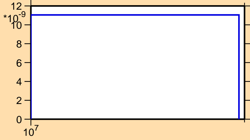
\sigma vs. E for ^{73}\text{Cu}(n,nt)
