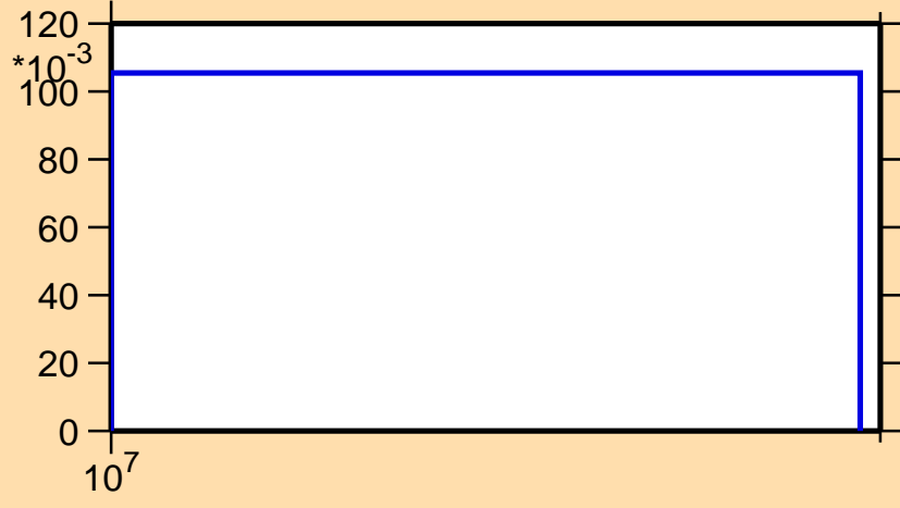
\sigma vs. E for ^{73}\text{Cu}(n,3n)
