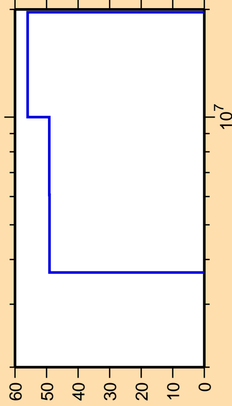
\Delta\sigma/\sigma vs. E for ^{74}\text{Cu}(n,n_1)
