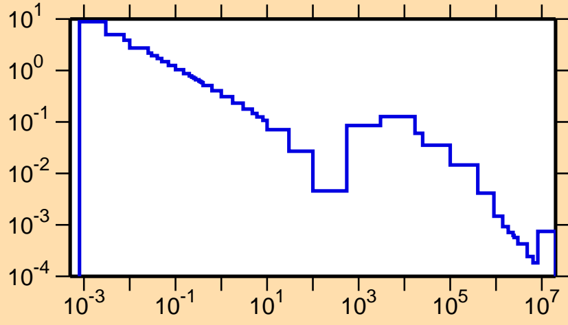
\sigma vs. E for ^{74}\text{Cu}(n,\gamma)
