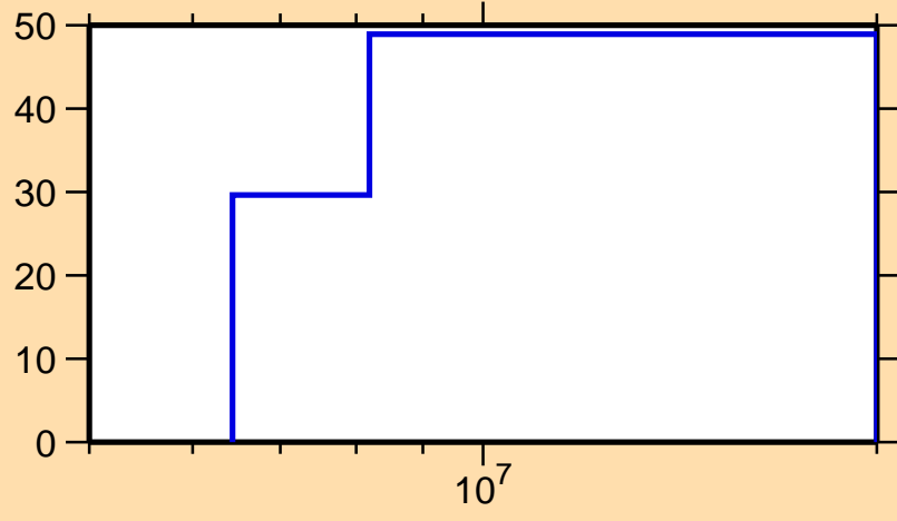
\Delta\sigma/\sigma vs. E for ^{74}\text{Cu}(n,ncont.)
