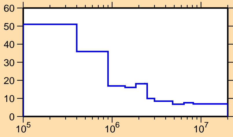
\Delta\sigma/\sigma vs. E for ^{74}\text{Cu}(n,n\text{onel.})
