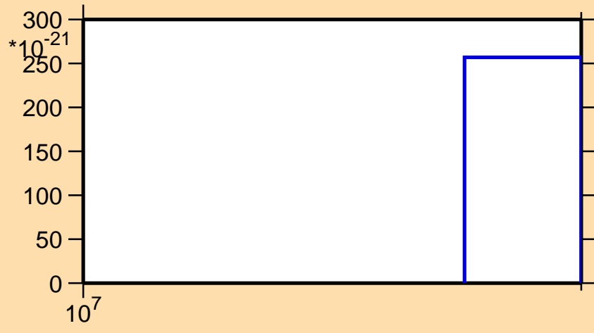
\sigma vs. E for ^{75}\text{Cu}(n,2n\alpha)
