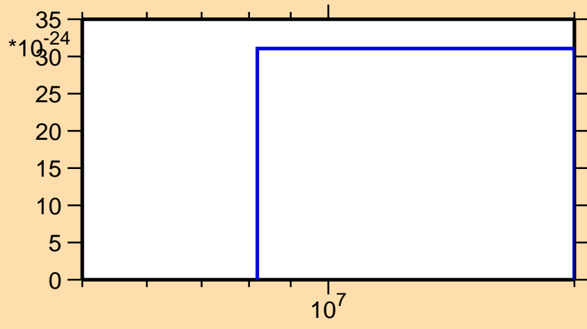
\sigma vs. E for ^{75}\text{Cu}(n,2np)
