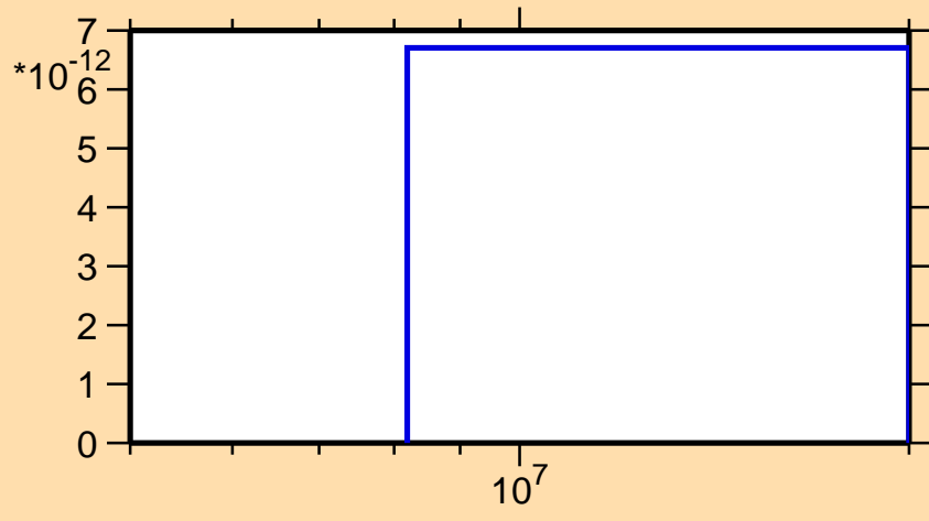
\sigma vs. E for ^{75}\text{Cu}(n,nd)
