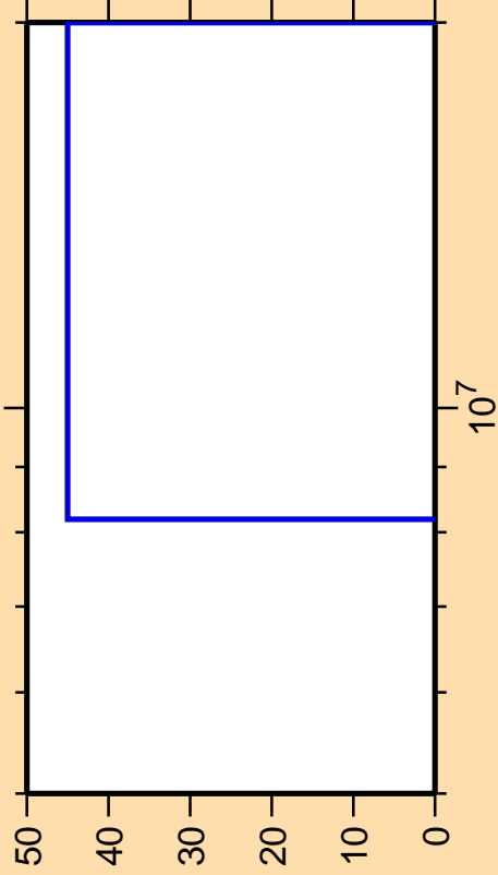
\Delta\sigma/\sigma vs. E for ^{75}\text{Cu}(n,nd)
