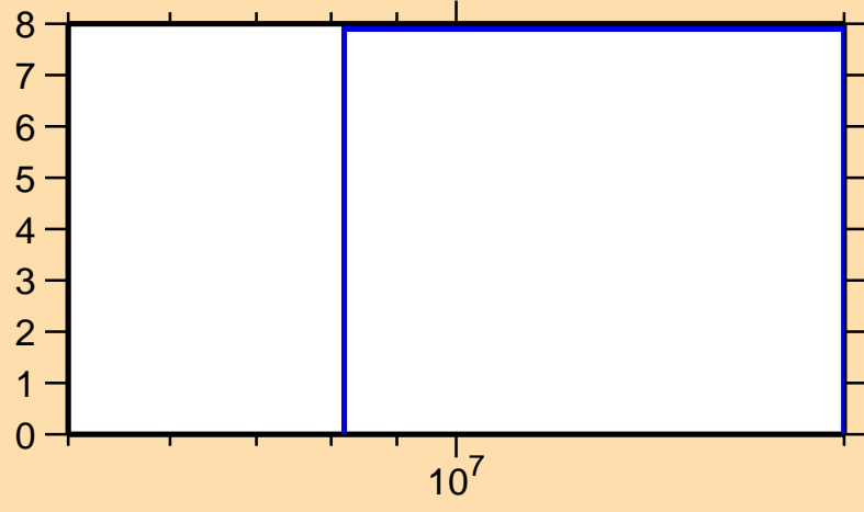
\Delta\sigma/\sigma vs. E for ^{76}\text{Cu}(n,el.)
