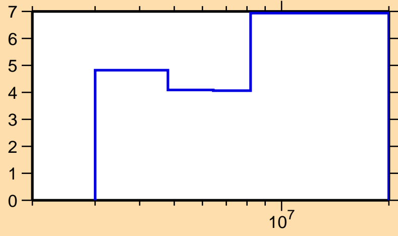
\Delta\sigma/\sigma vs. E for ^{76}\text{Cu}(n,\text{tot.})
