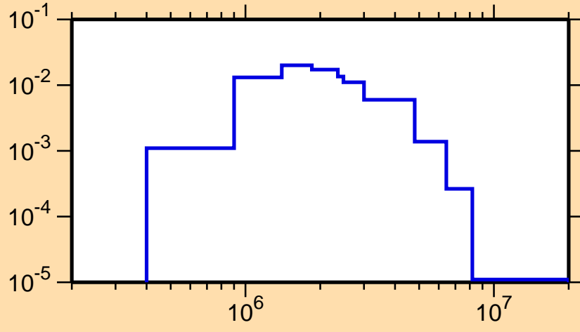
\sigma vs. E for ^{76}\text{Cu}(n,n_4)
