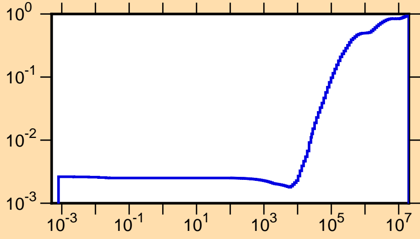
\mu vs. E for ^{255}
